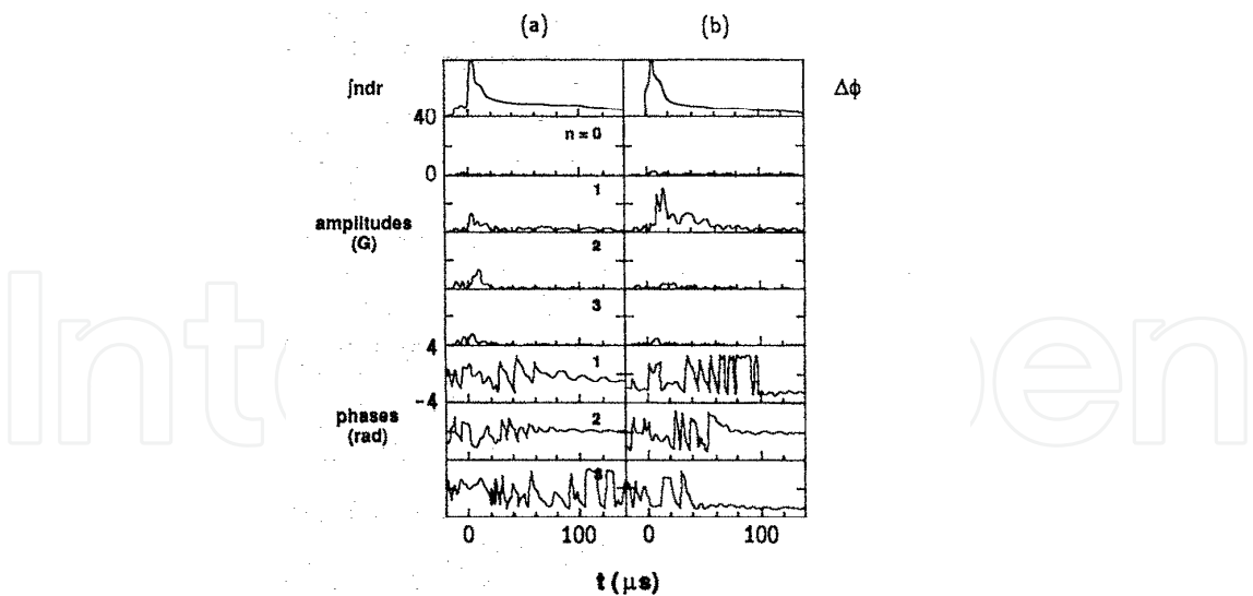
Fig. 8. Toroidal Fourier analysis of the B_0 for bad confinement. The Fourier amplitudes and phases are shown as functions of time for (a) even and (b) odd components The top trace of (a) is a line-integrated electron density and (b) diamagnetism.
