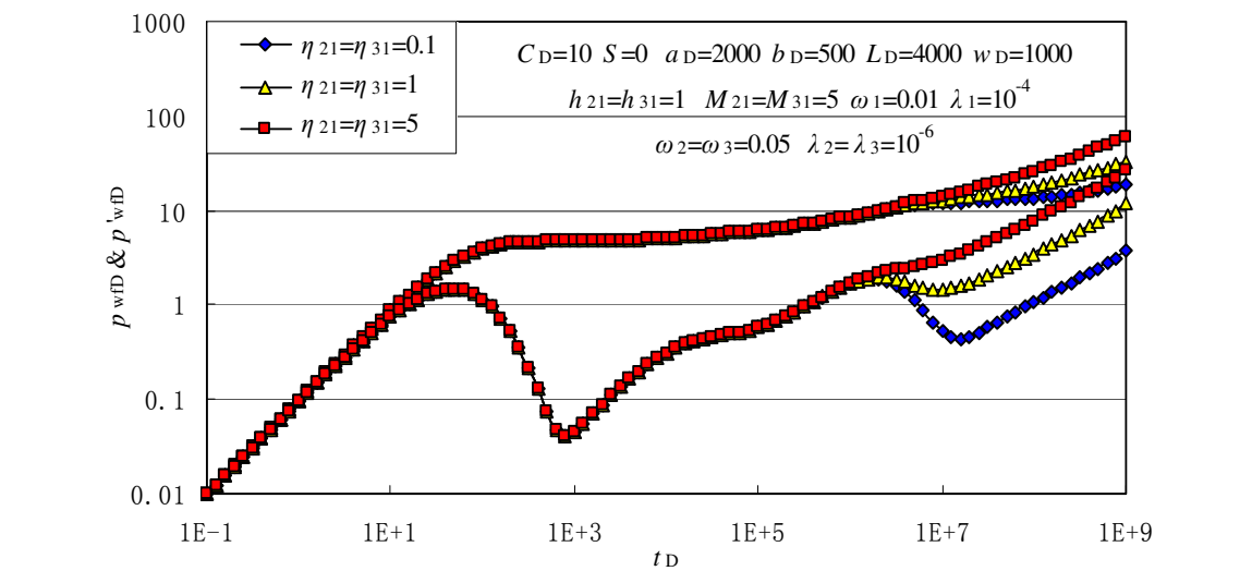
Fig. 6. Effect of transmissibility ratio on pressure responses for a well in a three-zone linear composite dual-porosity reservoir ( \eta_{21}=\eta_{31} )
