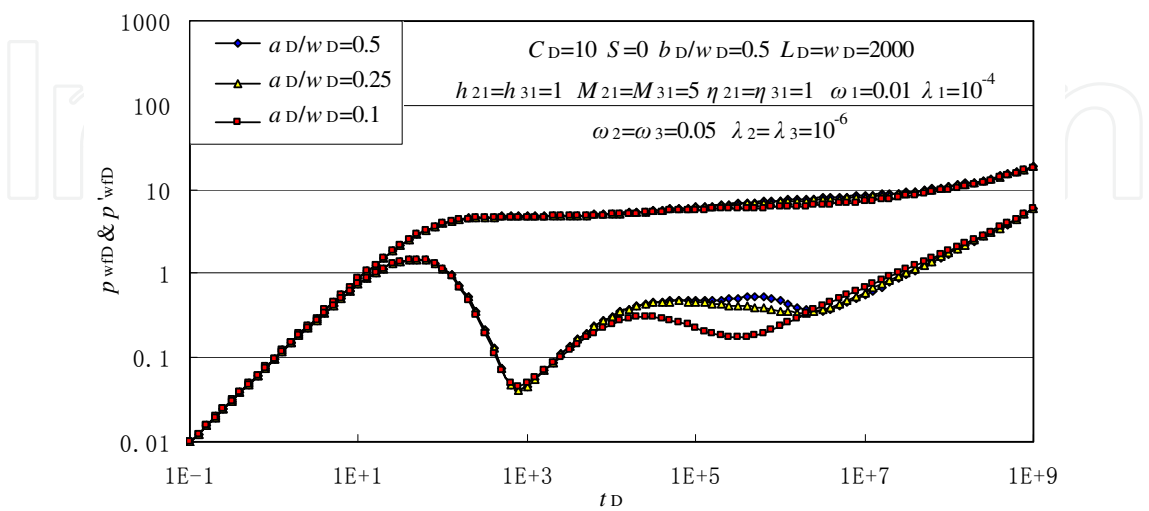
Fig. 7. Effect of well location ( a_D ) on pressure responses for a well in a three-zone linear composite dual-porosity reservoir
