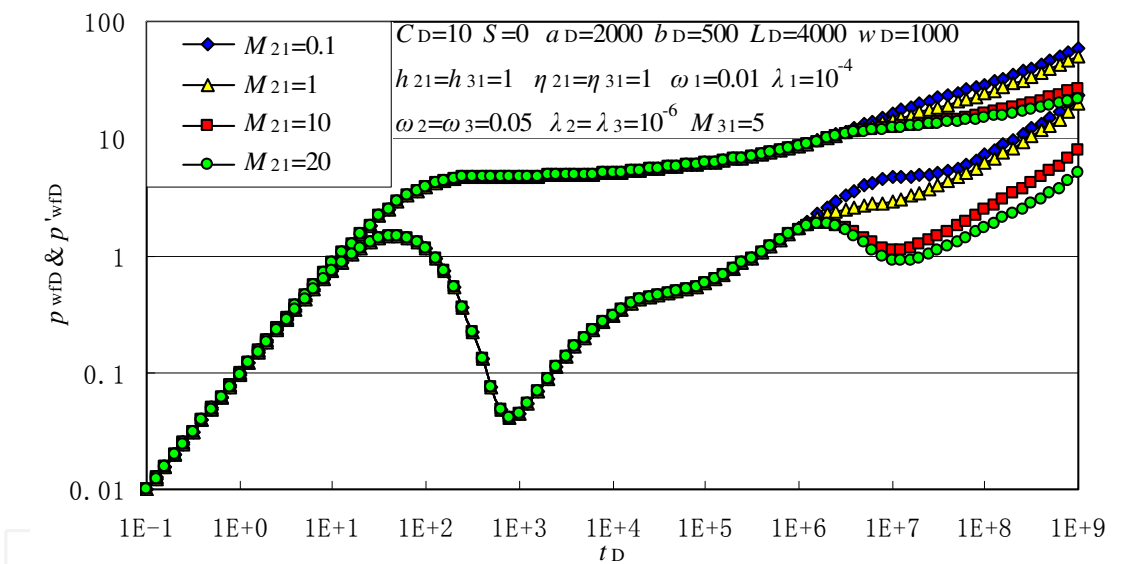
Fig. 5. Effect of mobility ratio on pressure responses for a well in a three-zone linear composite dual-porosity reservoir ( M_{21} \neq M_{31} )
