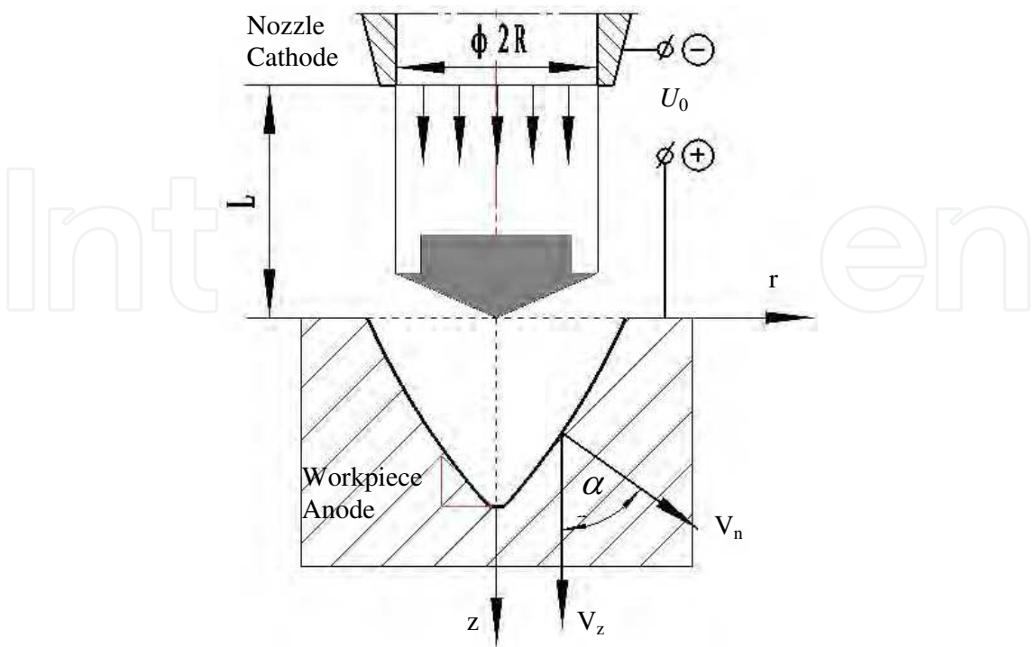
Fig. 11. Schematic diagram of the model for JECM process
