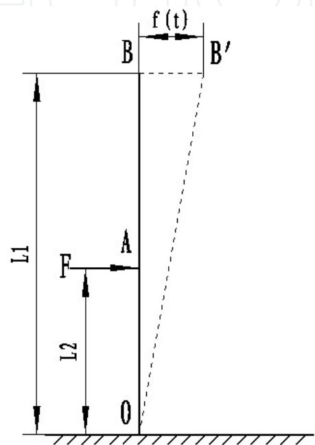
Fig. 6. Schematic diagram of vibrating cantilever
