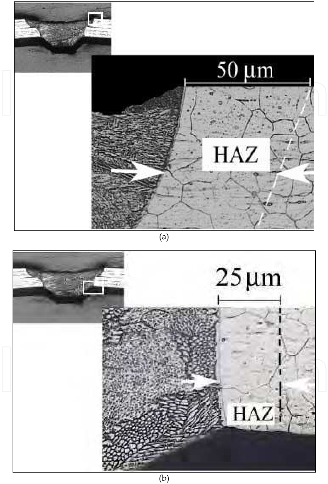
Fig. 13. Heat-Affect Zone of the top foil (a) and bottom foil (b) of the specimen welded with 2.25 J. (Ventrella, 2010)
