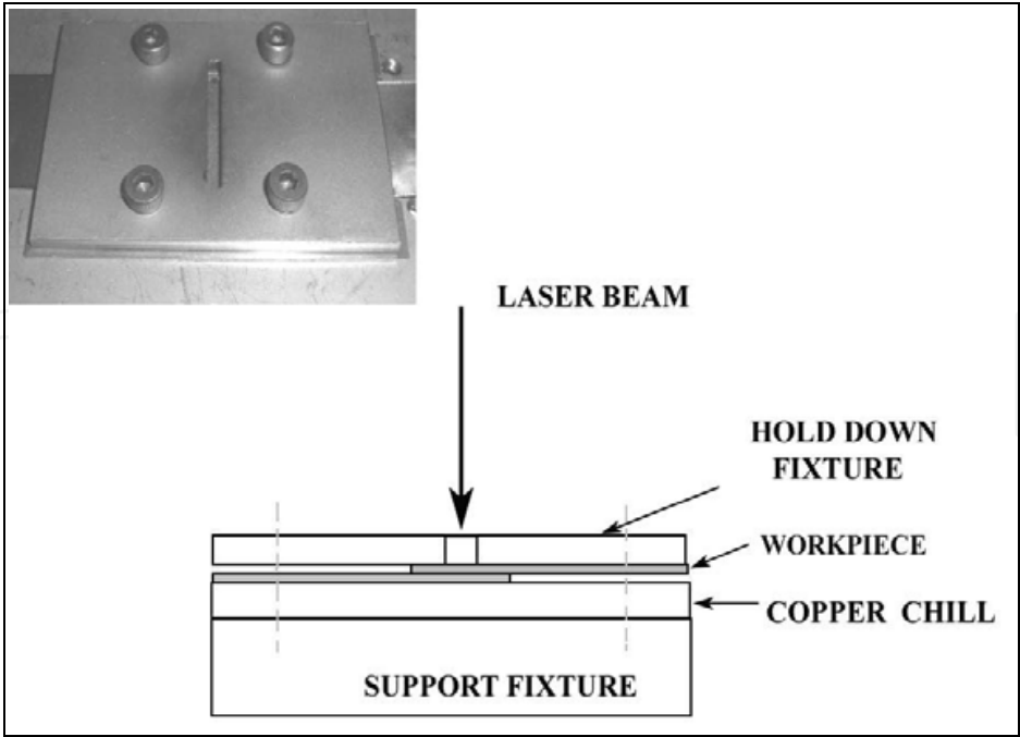
Fig. 5. Schematic of the hold-down fixture developed to hold the thin foils.
