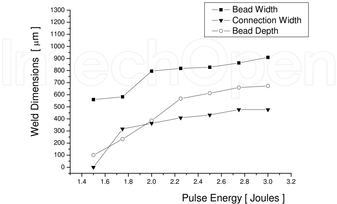
Fig. 11. Weld dimension versus pulse energy [ E_p ] of thin foil/thick sheet lap joints made with pulsed Nd:YAG laser welding with different pulse energies [ E_p ].
