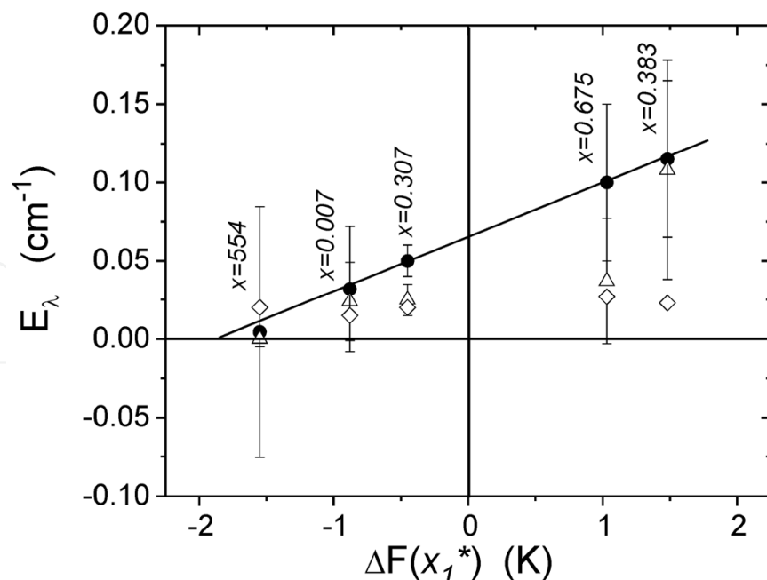
Fig. 11. Average light extinction for three \lambda within UV (●), Vis (△) and NIR (◇) spectral regions measured in ser.1-optical windows, finished from the lowest cylindrical section of the five representative boules vs. the difference in stability function values at coordinates corresponding respectively to upper and lower windows plane sections.
