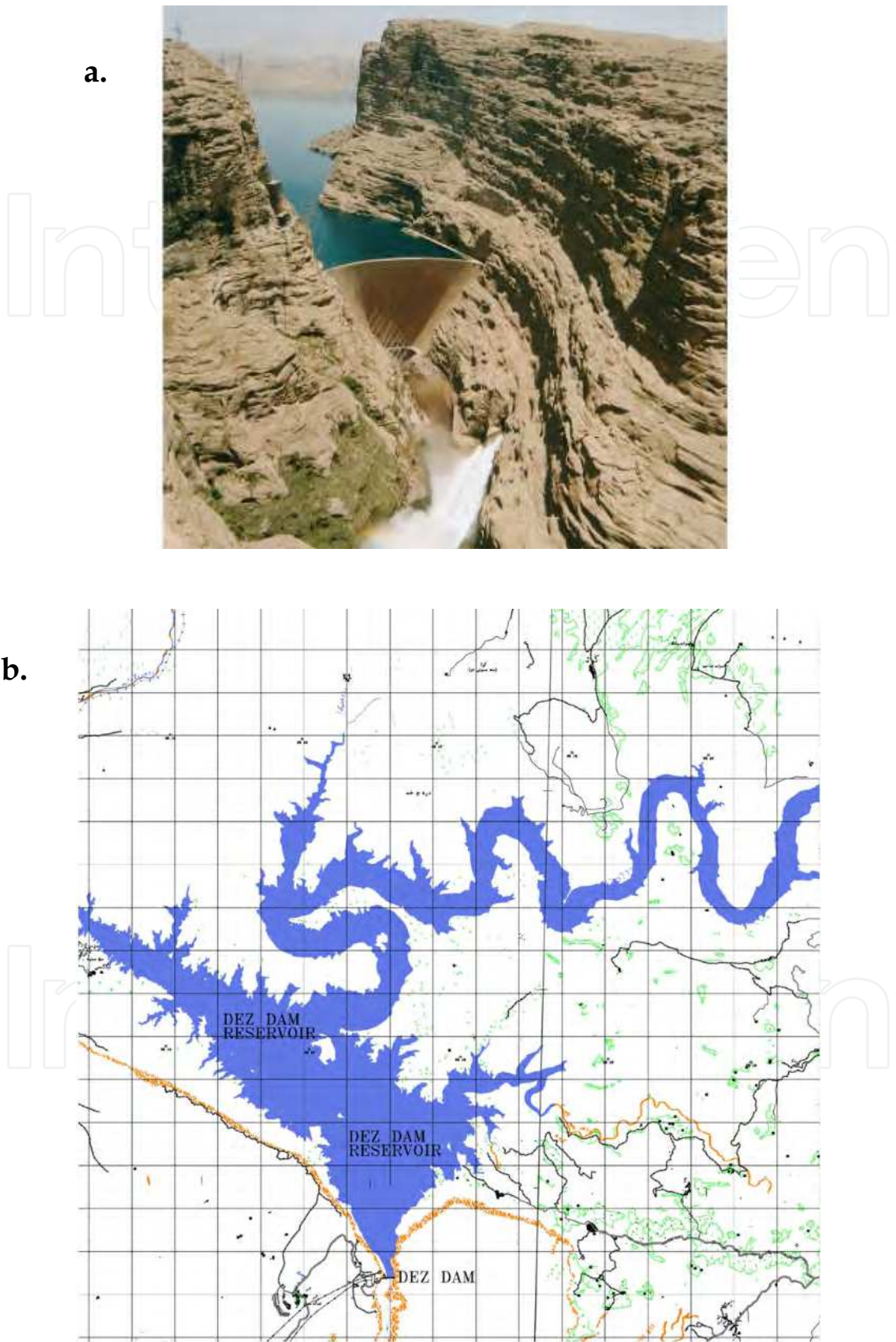
Fig. 2. (a) Photo of Dez Dam Project, (b) A plan view of Dez reservoir
