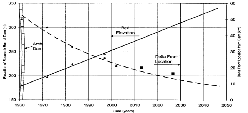
Fig. 7. Progressing Rate of delta front and increasing rate of bed elevation (near Dez dam) versus time based on Longitude profiles of Dez reservoir thalweg in different years.
