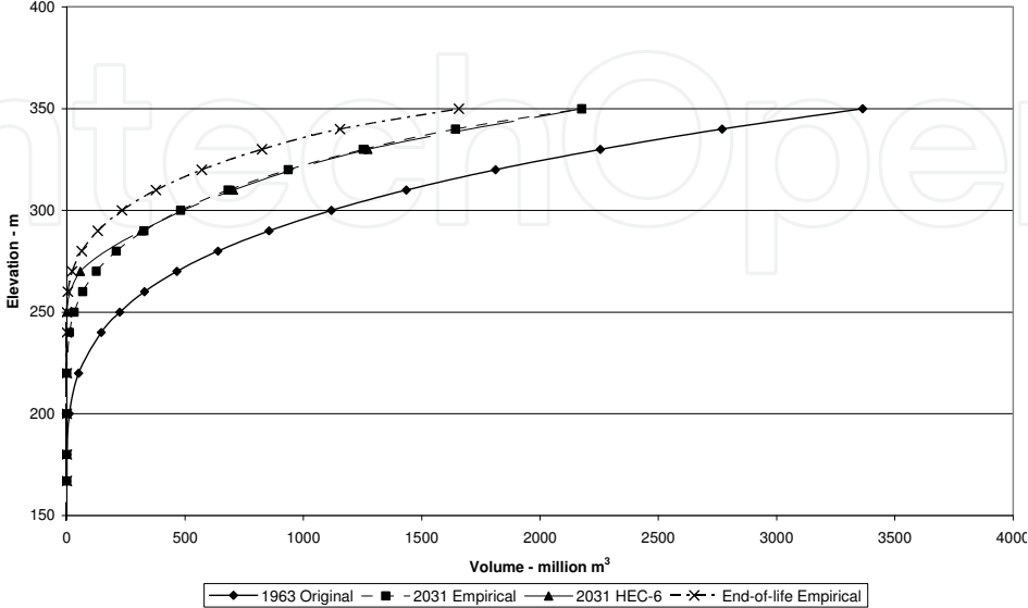
Fig. 8. End of Dez reservoir life volume elevation curve.
