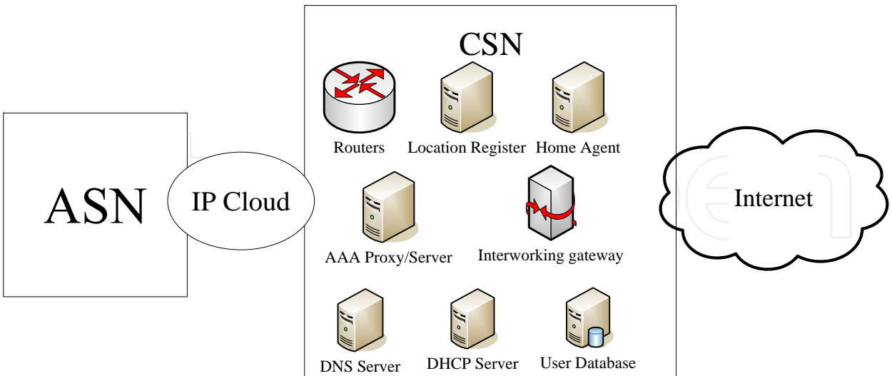
Fig. 1. CSN connection modules
