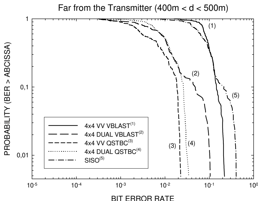
Fig. 19. Complementary cumulative distribution function of the BER far from the transmitter and for a fixed transmitting power (Sanchis-Borras et al., 2010).
