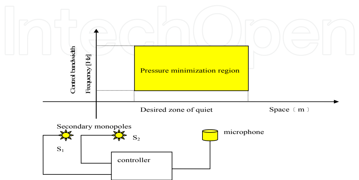
Fig. 3. Configuration of acoustic pressure minimization over space and frequency with a two-channel feedback system.
