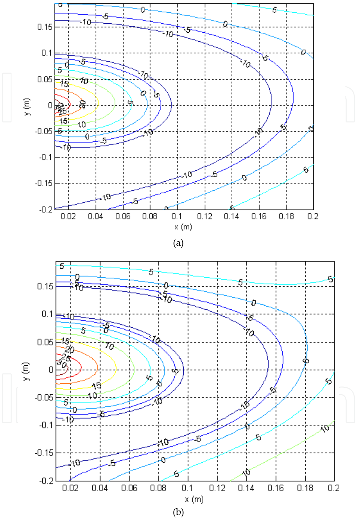
Fig. 10. Attenuation contour in decibels on x-y plane for the two-channel system with two FIR filters having 64 coefficients without constraints. (a) 400 Hz. (b) 600Hz.
