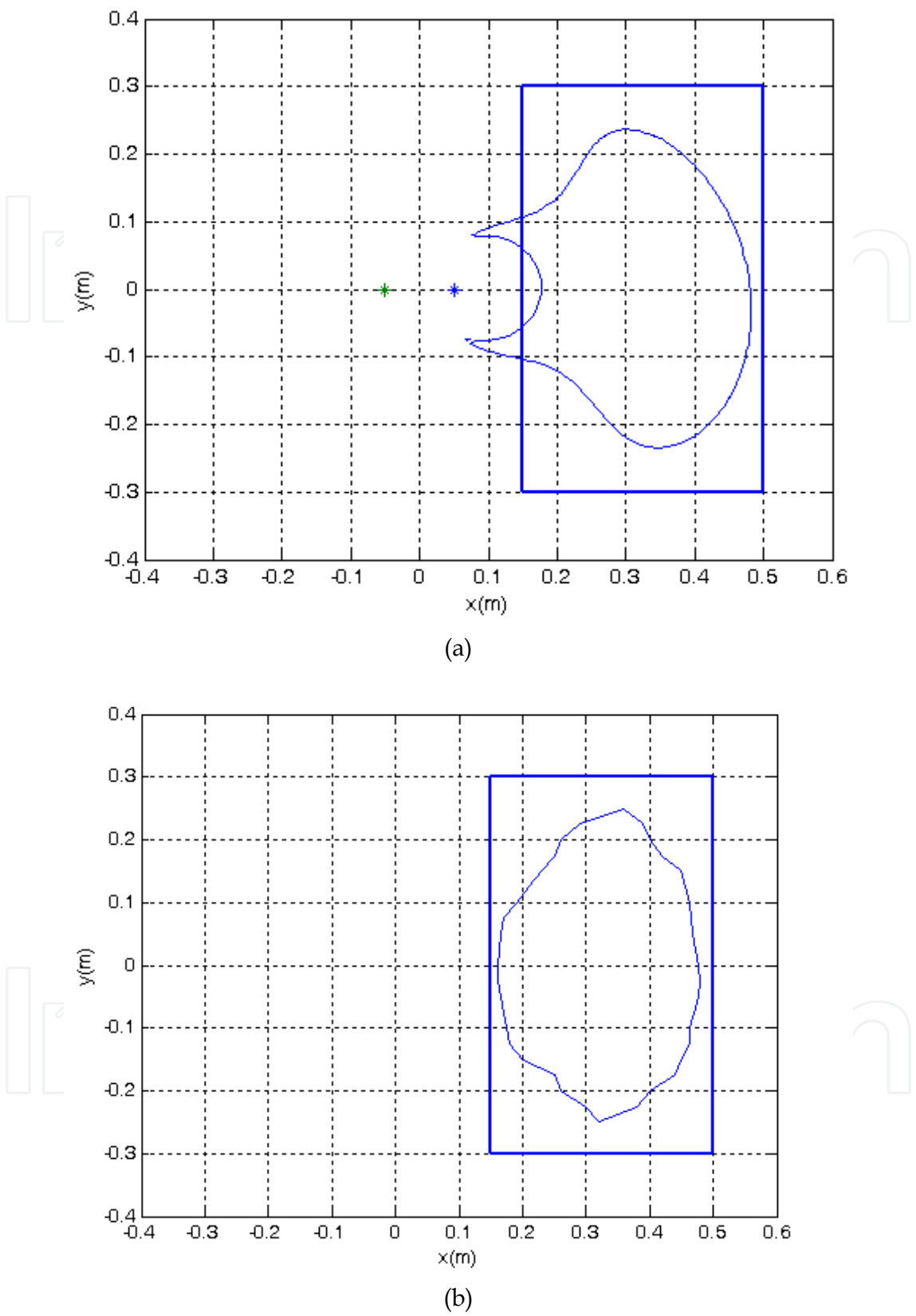
Fig. 16. The 10 dB reduction contour of the average zones of quiet created by two secondary sources located at positions (0.05, 0) and (-0.05, 0) using \infty -norm pressure minimization for 108Hz of diffuse primary fields. (a) Computer simulations. (b) Experiments.
