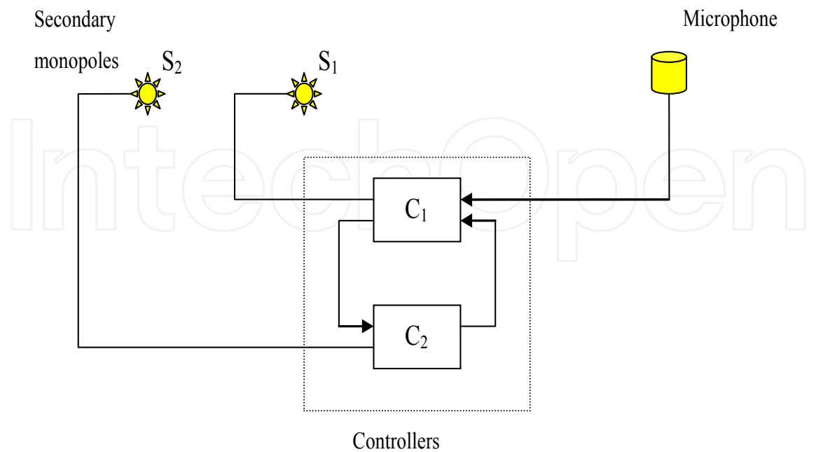
Fig. 4. Two-channel feedback control system used to control broad-band diffuse fields.
