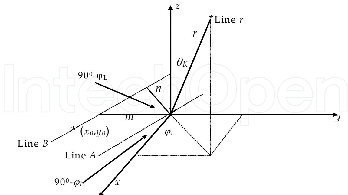
Fig. 1. Definition of spherical co-ordinates r , \theta , \varphi for an incident plane wave travelling along line r direction.
