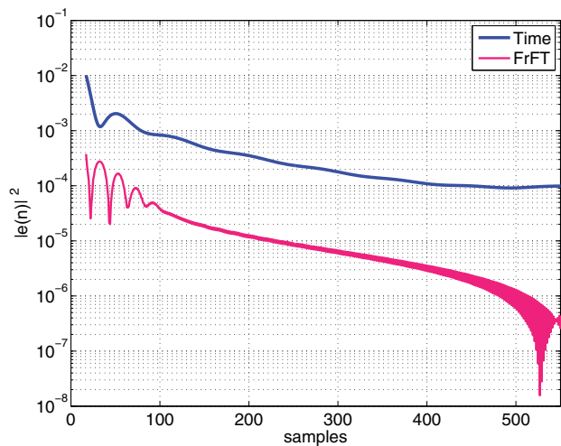
Fig. 14. Convergence analysis for both time and FrFT domain adaptive filtering.
