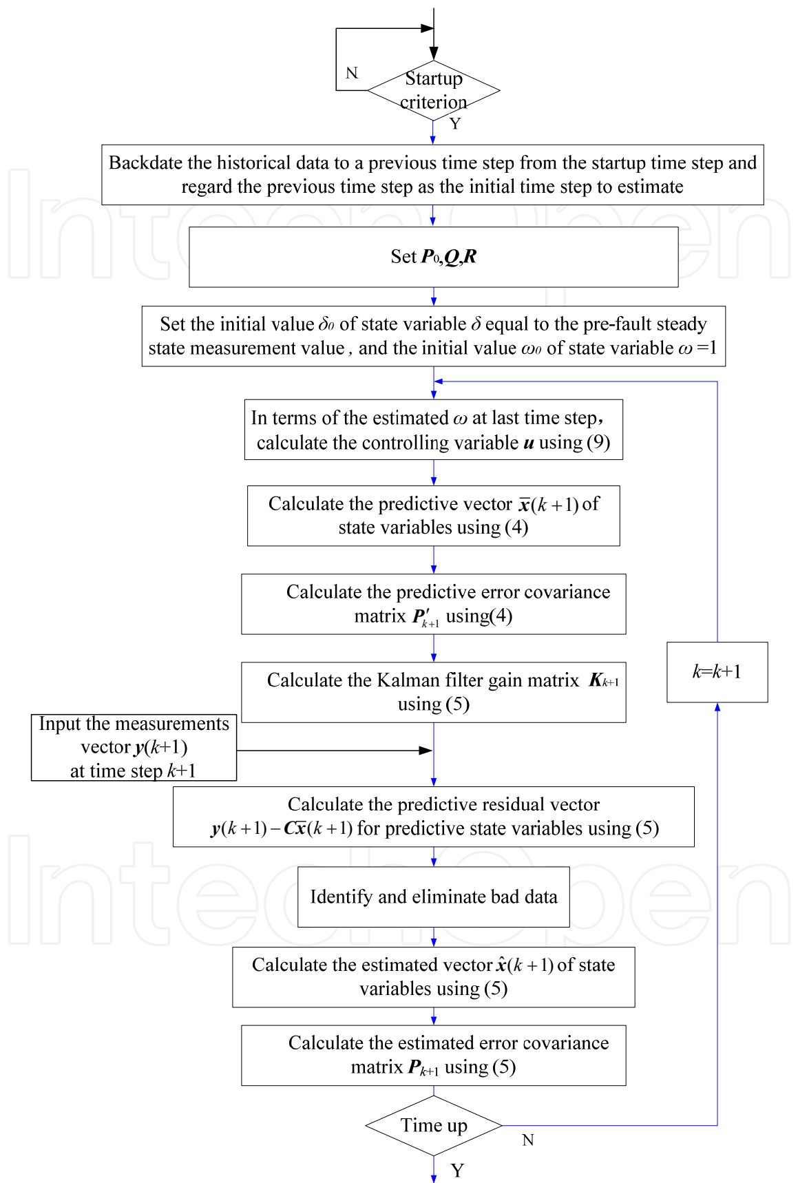
Fig. 1. Flow chart of the proposed dynamic state estimator.
