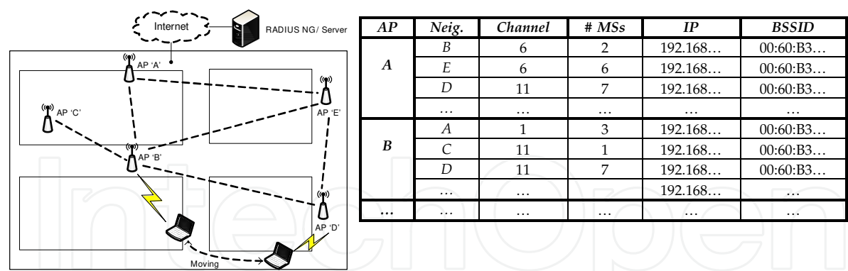
Fig. 5. The NG-based handover architecture
