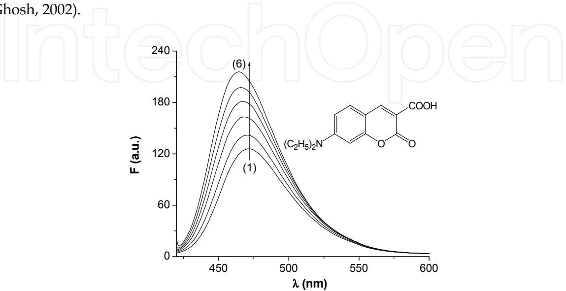
Fig. 3. The fluorescence spectrum of DEAC ( 2\times 10^{-6} M) in the presence of increasing amounts of \gamma -CD. \lambda_{ex} = 410 nm.
