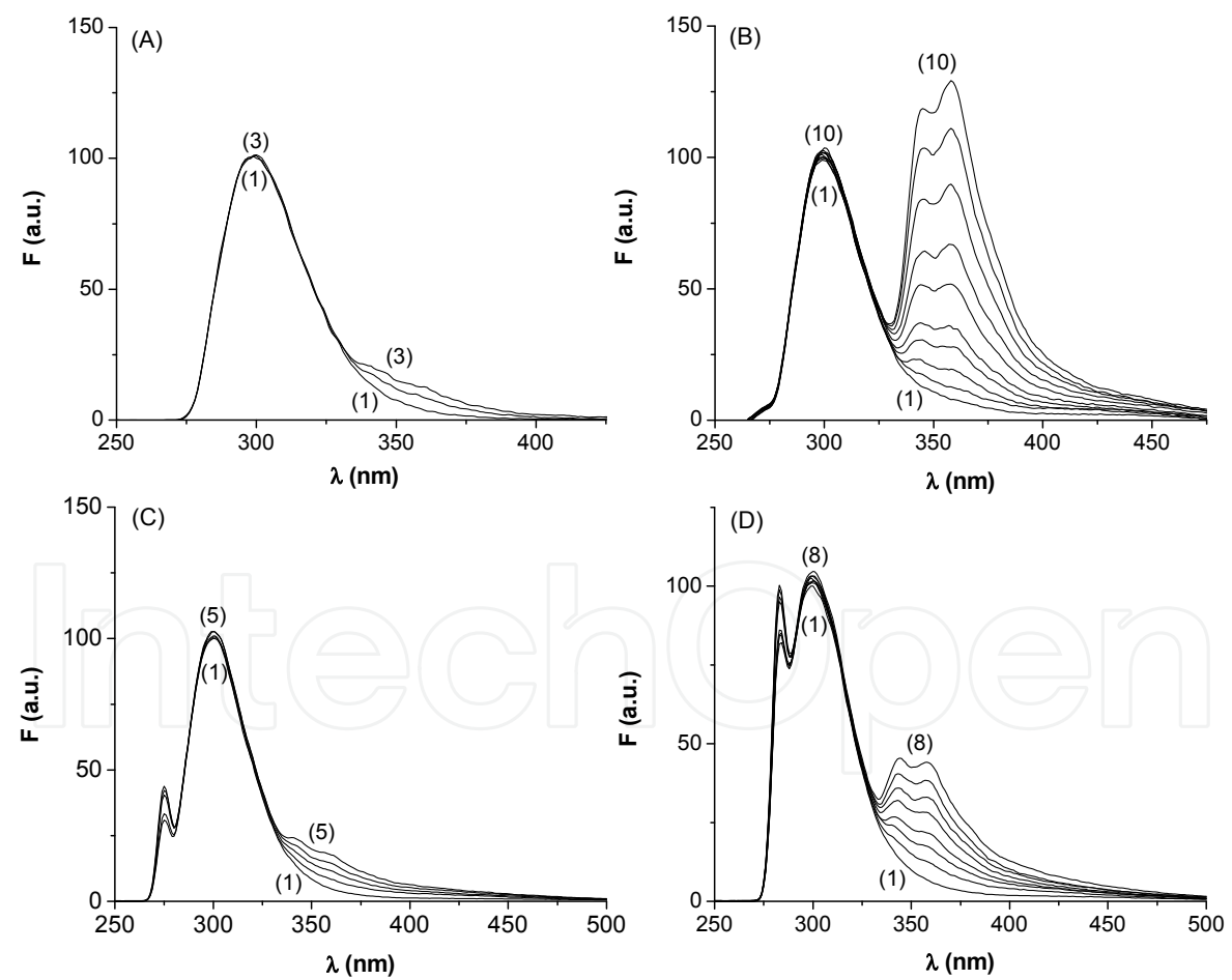
Fig. 11. The fluorescence spectrum of atenolol ( 2 \times 10^{-5} M in methanol:water 1:9 v:v) in absence (1) and presence (2-10) of increasing amounts of \alpha -CD (up to 7.4 \times 10^{-4} M), at various \lambda_{ex} (nm): (A) 225, (B) 250, (C) 275 and (D) 282.
