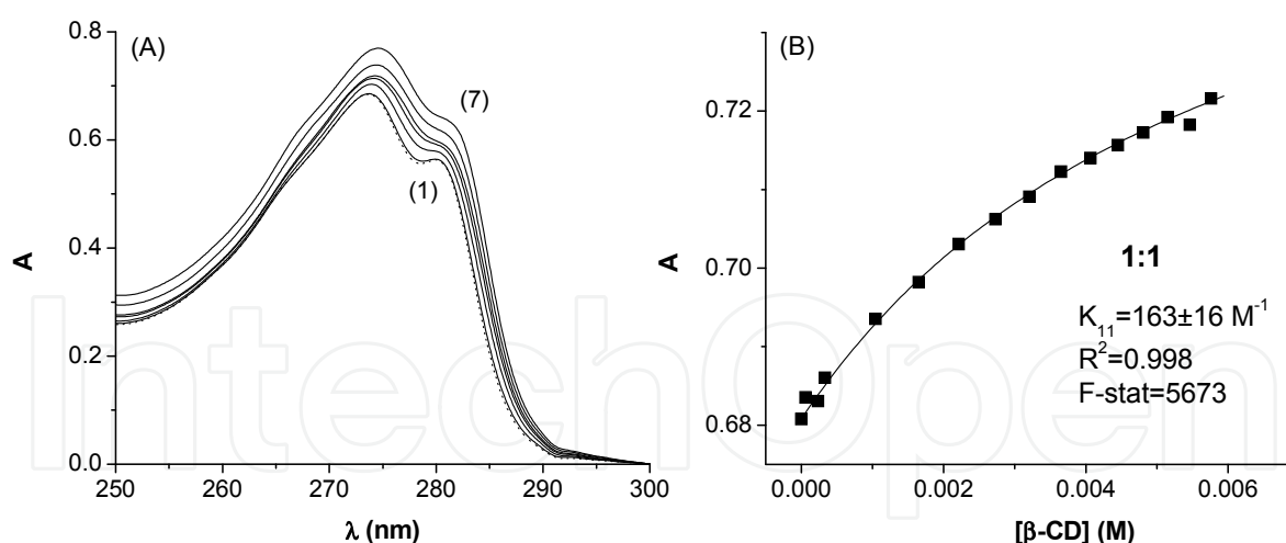
Fig. 16. (A) The absorption spectra of atenolol (5 × 10 -4 M in pH 7.4 phosphate buffer) in absence (1) and presence (2–7) of increasing concentrations of \beta -CD (up to 2 × 10 -2 M). (B) Determination of the stoichiometry and association constant of the atenolol- \beta -CD complex.
