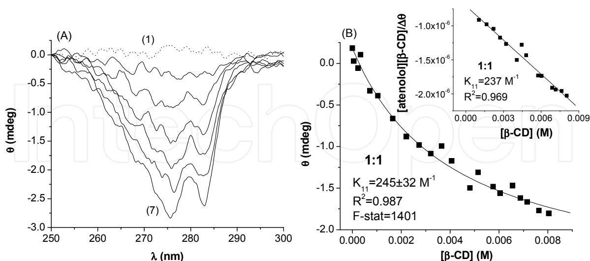
Fig. 15. (A) The circular dichroism spectra of atenolol (5 × 10 -4 M in pH 7.4 phosphate buffer) in absence (1) and presence (2–7) of increasing concentrations of \beta -CD (up to 2 × 10 -2 M). (B) Determination of the stoichiometry and association constant of the atenolol- \beta -CD complex.
