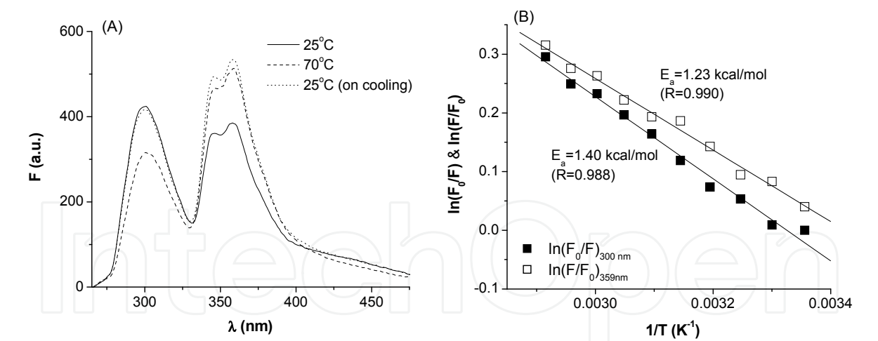
Fig. 13. The temperature dependence of the fluorescence intensity of the atenolol- \gamma -CD system in methanol:water 1:9 v:v (A) and the activation energies of the respective processes (B). \lambda_{ex} = 250 nm.
