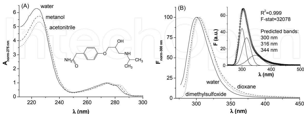
Fig. 8. Absorption (A) and fluorescence (B) spectra of atenolol in different solvents. Inset: Deconvolution of the fluorescence spectrum of atenolol in dimethylformamide. \lambda_{\text{ex}} = 275 \text{ nm} .
