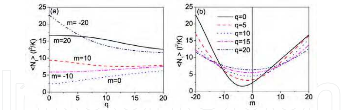
Fig. 8. Averaged first normal stress difference. Adapted from Guillen and Mendoza 2007.
