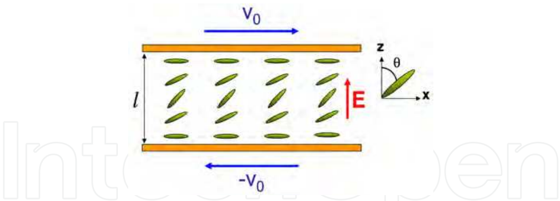
Fig. 9. Schematics of a homogeneous cell subjected to a normal electric field and a shear stress. Adapted from Medina and Mendoza 2008.
