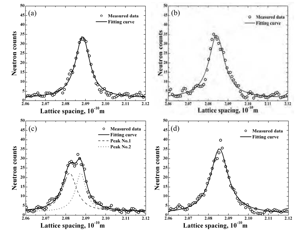
Fig. 10. Austenite (111) peaks and fitting results: (a) non-splitting, \varepsilon=0.0 ; (b) peak shift, \varepsilon=0.05 ; (c) peak splitting at \varepsilon=0.15 ; (d) disappearance of peak splitting at \varepsilon=0.33 .
