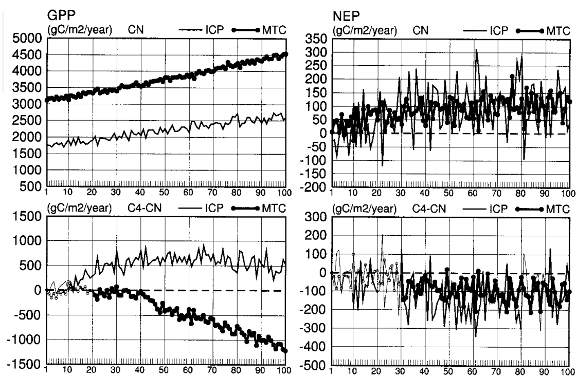
Fig. 7. Temporal distributions of the annual mean values of GPP (left) and NEP (right) (gC m -2 year -1 ) for the 100-year simulations. The horizontal axes indicate the model years. The solid lines are for the Indochina peninsula area (ICP), and the lines with circle are for the Maritime Continent area (MTC). Top panel is for the control, and bottom panel is for the differences between the control and the C4 experiment (C4 - CN). In the bottom panel, thick lines for each area indicate statistically significant differences in each 10-year period.
