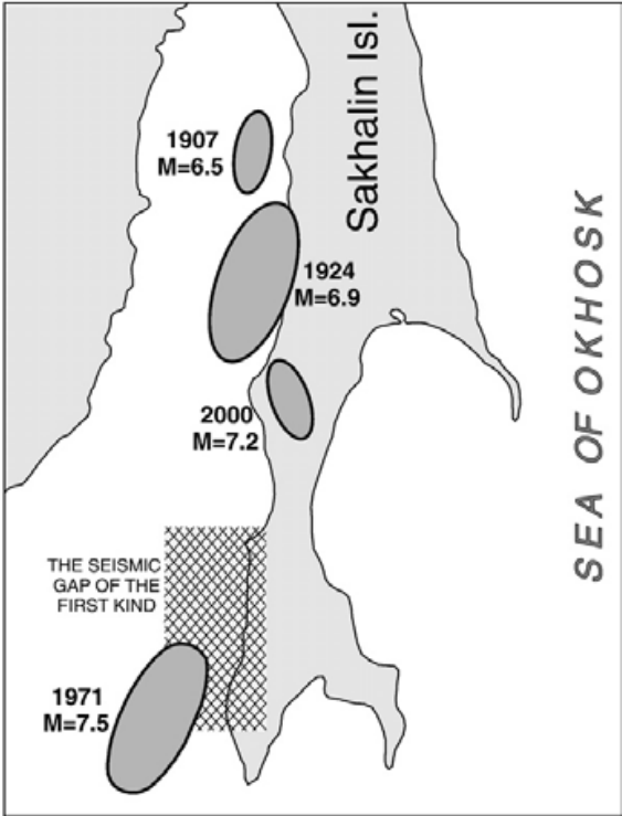
Fig. 16. Sources of large earthquakes at the western coast of Sakhalin Island (grey ovals) and the approximate location of the seismic gap of the first kind (hatched rectangle).
