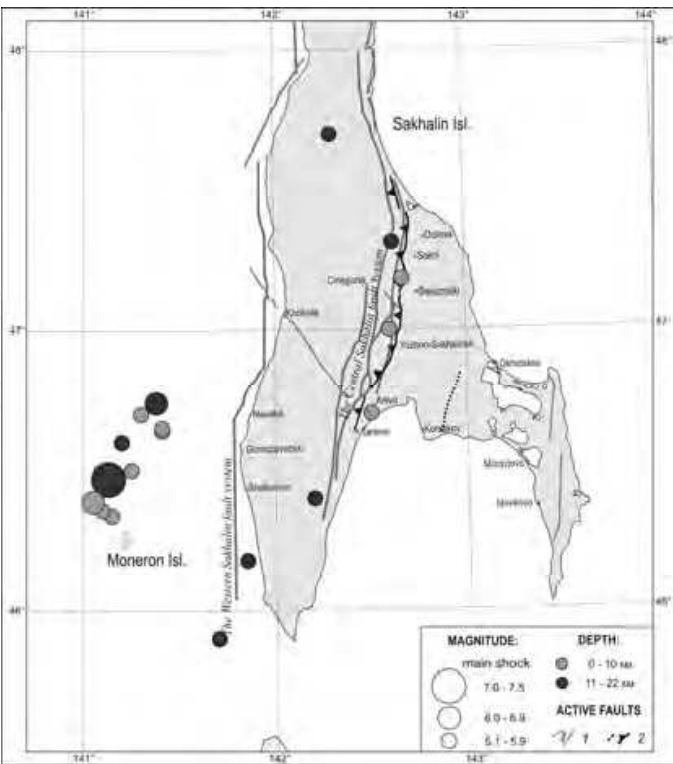
Fig. 15. Map of crust earthquake M > 5.0 epicenters of southern Sakhalin, 1906–2005, and the main fault zones. Notes: The active faults are plotted according to M.I. Streltsov of IMG&G FEB RAS, Yuzhno-Sakhalinsk (1) and A.I. Kozhurin, of GIN AS, Moscow (2).
