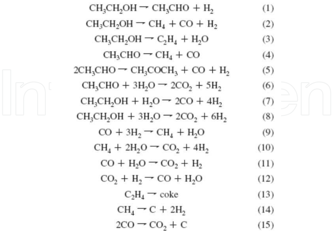
Fig. 26. Reactions Involved in Ethanol Steam Reforming over Co-Based Catalysts (Song et al., 2010)
