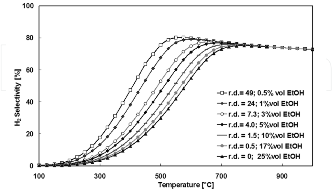
Fig. 9. H 2 selectivity as a function of temperature at different dilution ratios
