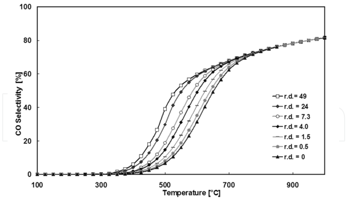
Fig. 11. CO selectivity as a function of temperature at different dilution ratios
