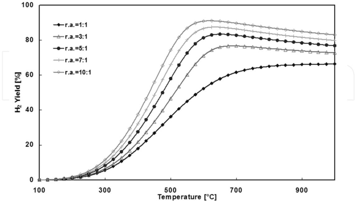
Fig. 8. \text{H}_2 yield as a function of temperature at different water to ethanol molar ratios
