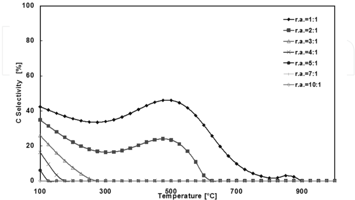
Fig. 7. C selectivity as a function of temperature at different water to ethanol molar ratios.
