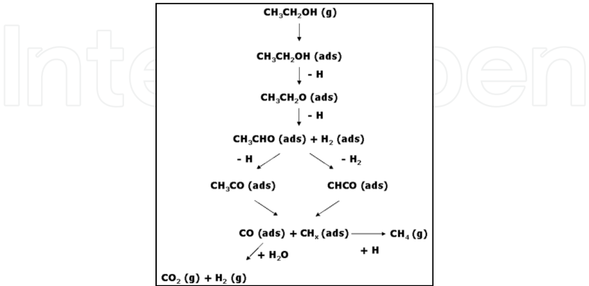
Fig. 20. Scheme of the surface reaction mechanism proposed (Ciambelli et al., 2010b)
