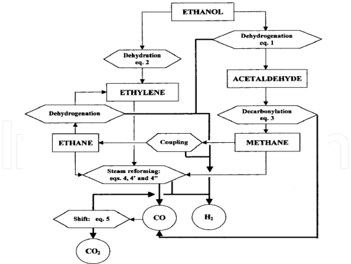
Fig. 16. Pathways for the steam reforming of ethanol over Rh/ Al 2 O 3 catalysts (Cavallaro, 2000)
