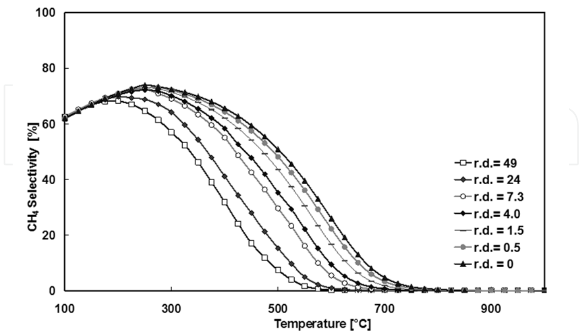
Fig. 10. CH 4 selectivity as a function of temperature at different dilution ratios
