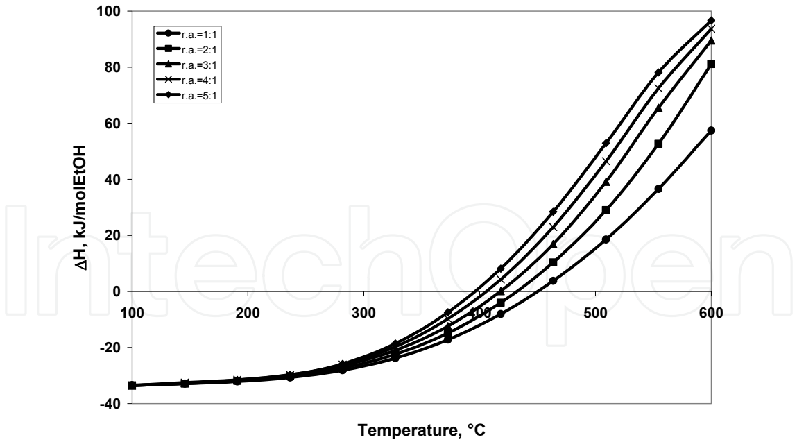
Fig. 15. Effect of temperature and water to ethanol and oxygen to ethanol molar ration on ΔH of reaction
