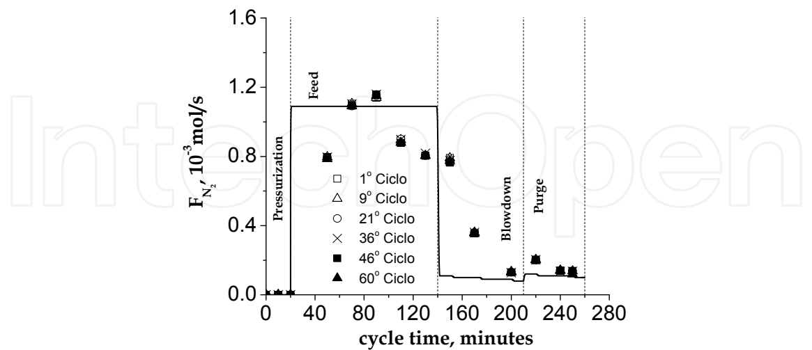
Fig. 7. Nitrogen molar flow rate as a function of cycle time. Experimental conditions: run 2. Solid line: first cycle simulation. Dashed line: CCS simulation.
