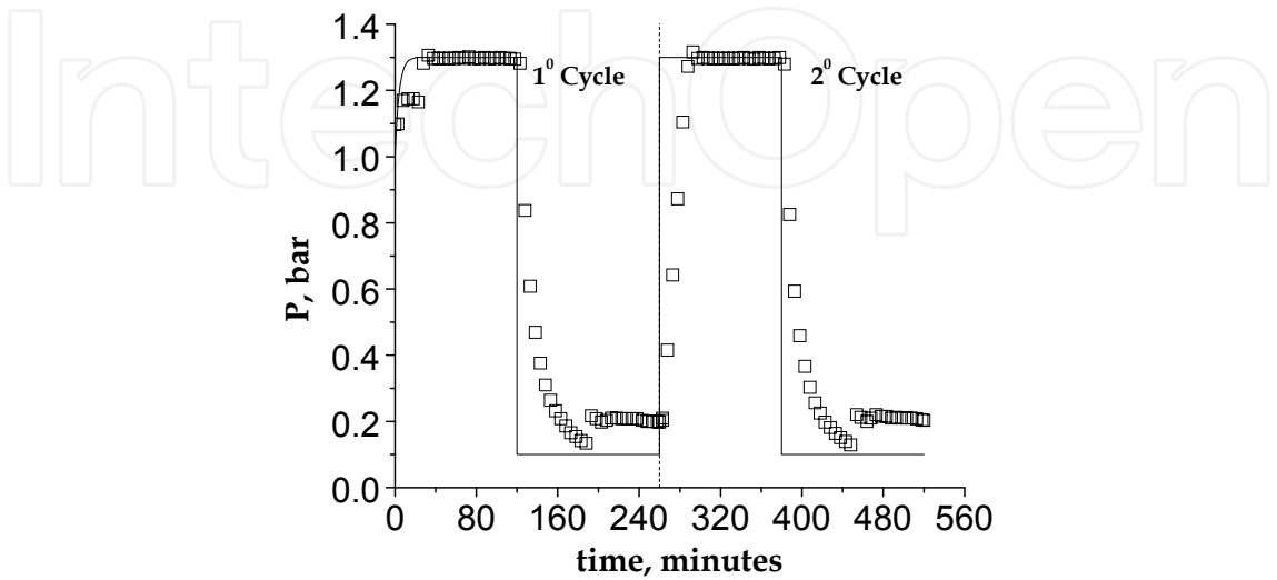
Fig. 5. Pressure change as a function of process time. Experimental conditions: run 1.
