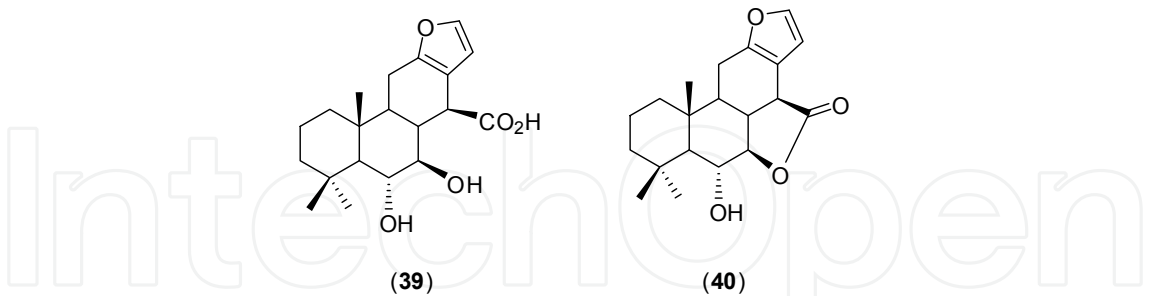
Fig. 10. Structure of diterpene (39) and its synthetic derivative (40).
