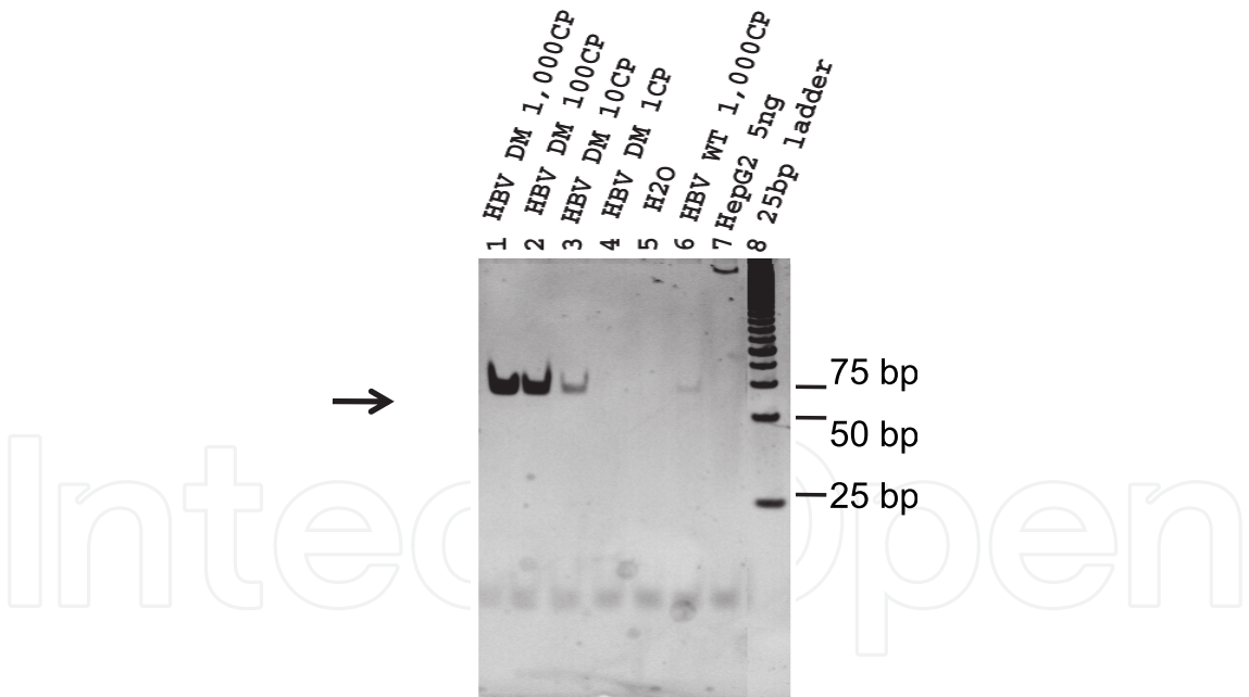
Fig. 5. Sensitivity and specificity of the HBVDM_40 assay. Serial 10-fold dilutions from 1 copy to 1000 copies of HBV 1762T/1764A double mutation positive control plasmid DNA and 1000 copies of the plasmid DNA containing HBV wild type sequences, 5 ng of HepG2 DNA, and H 2 O were subjected to the HBVDM_40 assay. PCR products of the second-step PCR were analyzed in 12% polyacrylamide gel, stained with ethidium bromide, and visualized by photographing under a UV-transilluminator. The location of an expected 62-bp amplicon is indicated by the arrow. The TrackIt™ 25 bp DNA Ladder was used to indicate molecular weight markers.
