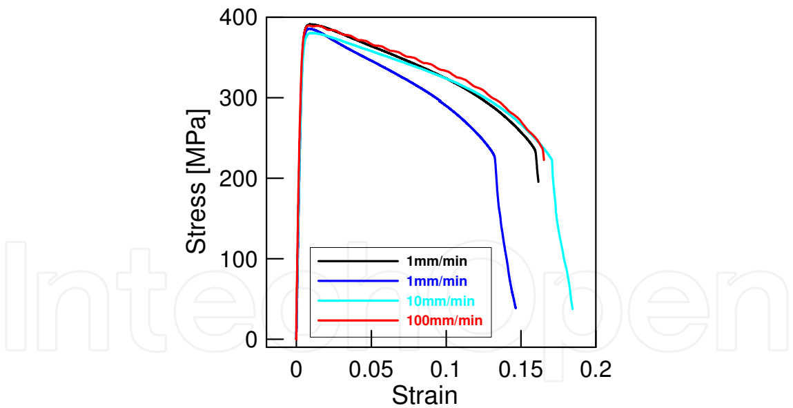
Fig. 5. Tensile diagrams of UFG Cu prepared by ECAP, route Bc
