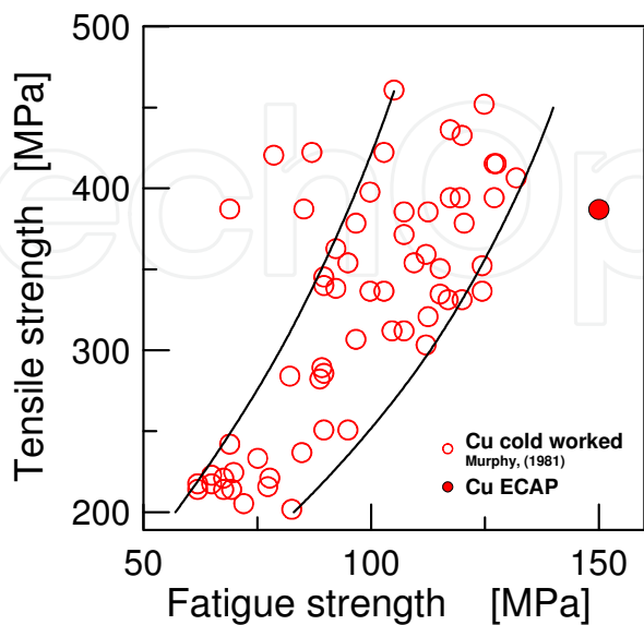
Fig. 8. Relation of tensile and fatigue strength for fatigue limit based on 10^8 cycles for cold worked Cu (Murphy, 1981) and UFG Cu
