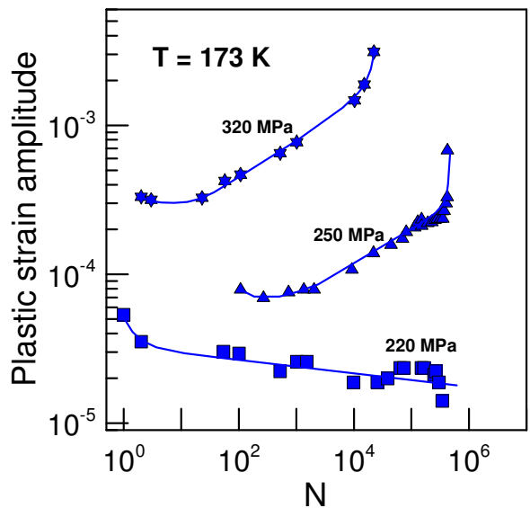
Fig. 20. Cyclic softening/hardening curves of UFG Cu loaded at temperature 173 K
