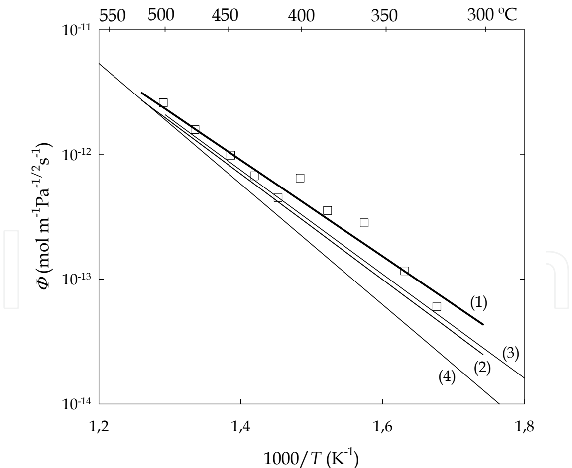
Fig. 7. Hydrogen permeability in PH-CuCrZr ELBRODUR® alloy compared with reference copper alloys: (1) ELBRODUR®, (2) GlidCop® Al25, (3) ELBRODUR-II, (4) pure Cu.
