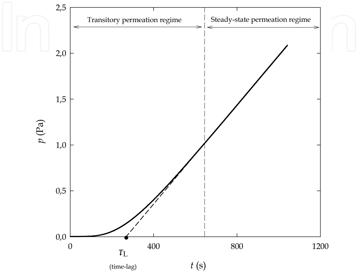
Fig. 3. Experimental permeation curve: transitory permeation regime and steady-state permeation regime. Definition of the time-lag.
