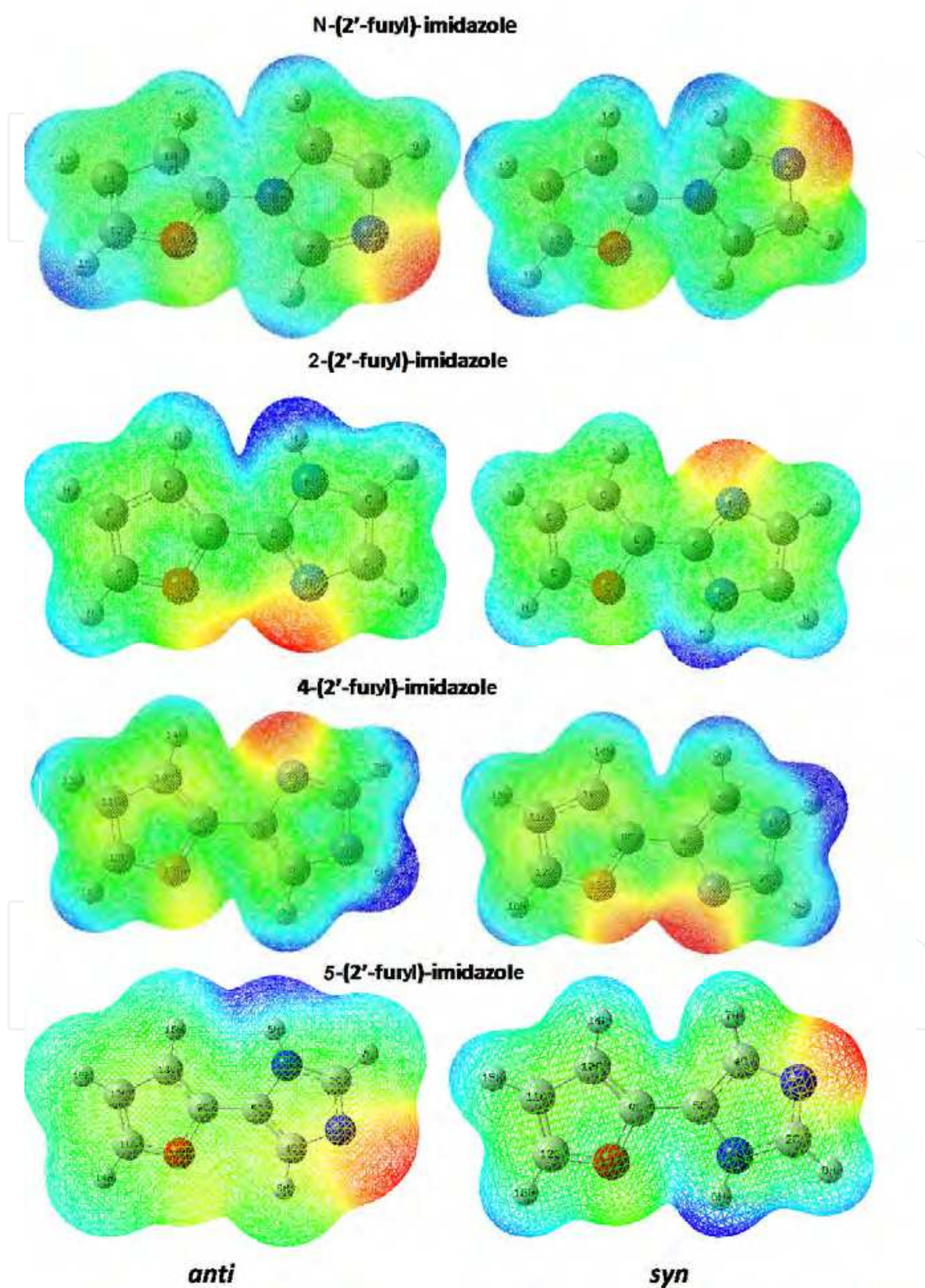
Fig. 3. Electrostatic Surface Potential calculated on the molecular surface of the conformers for all compounds of the series. Color, in u.a.: from red -0.103 to blue 0.103.
