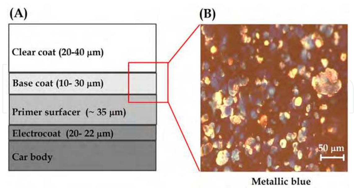
Fig. 1. (A) Schematic representation of the cross-section of a typical car coating and related layer thickness (in μm). (B) Optical micrograph of a metallic blue coating containing aluminium flakes and conventional absorption blue pigments in the base coat. Bright field illumination (20x).
