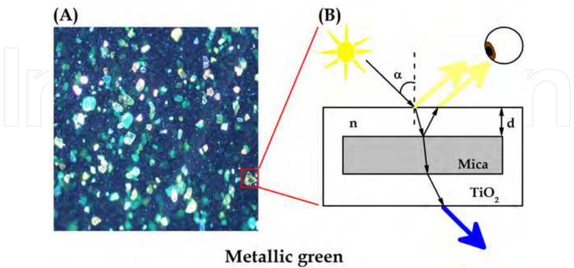
Fig. 2. (A) Optical micrograph of a metallic green coating containing greenish-yellowish interference pigments, aluminium flakes and opaque green absorption pigments. Darkfield illumination (20x). (B) Schematic representation of the cross-section of a mica flake coated by titanium dioxide (TiO 2 ) with thickness d and refractive index n .
