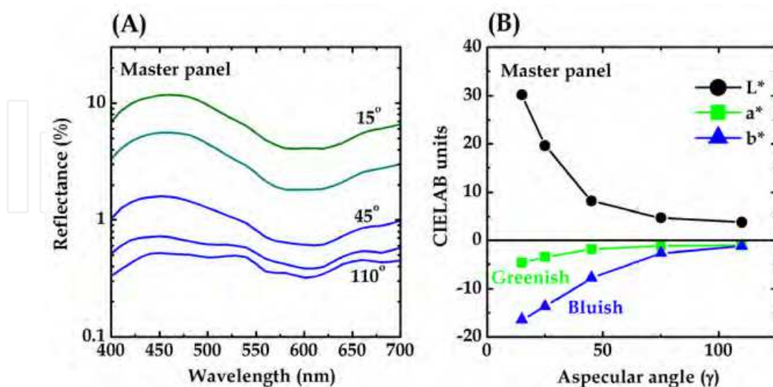
Fig. 8. (A) Reflectance spectra of a typical blue metallic coating at the aspecular angle \gamma of 15°, 25°, 45°, 75° and 110°. (B) CIE L^* , a^* and b^* colour coordinates calculated at different the aspecular angles. The reference illuminant was D65. Data indicate the master panel.
