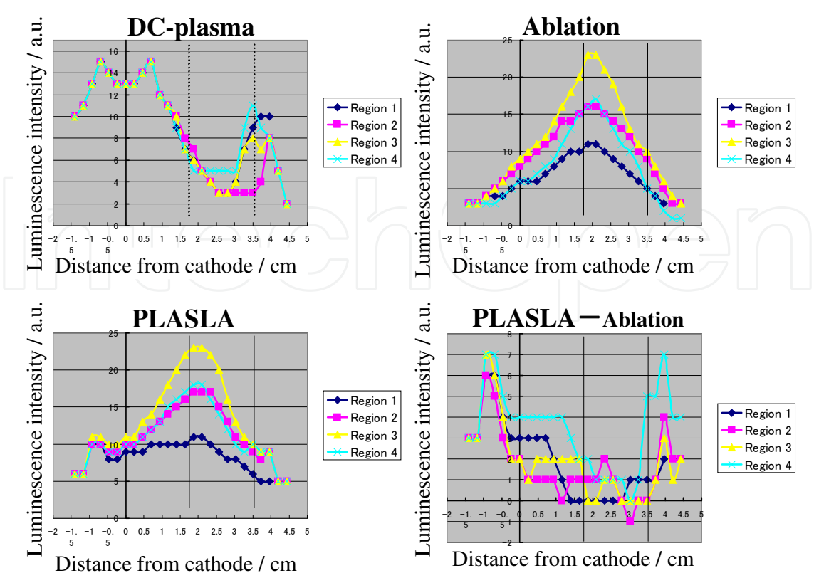
Fig. 6. Luminescence intensities between electrodes in DC-plasma, Ablation (CuF chemi-luminescence), PLASLA, and the difference in the luminescence intensity between the PLASLA and laser-ablation patterns.
