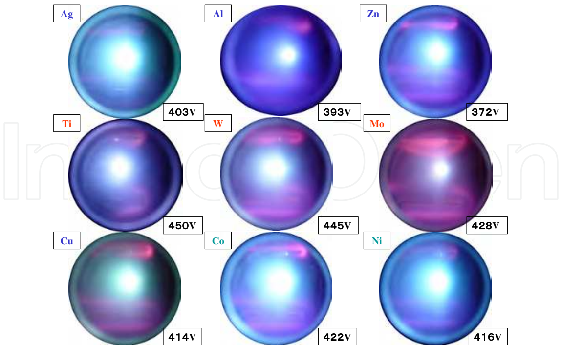
Fig. 3. PLASLA discharge patterns with various target metals. Metals and PLASLA potentials are indicated on the upper-left sides and lower-right sides of discharge images, respectively. The colours indicating metals are classifying them into groups: Group-1 is in blue, Group-2 in green, Group-3 in red.
