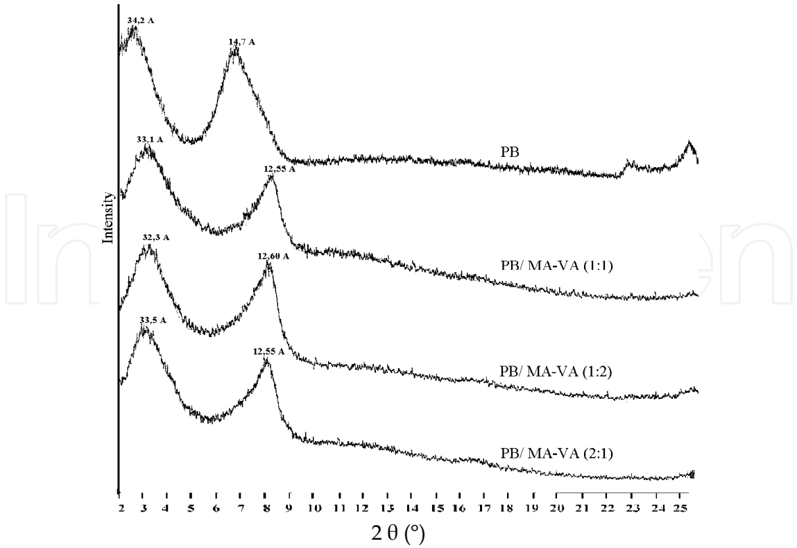
Fig. 8. X-ray diffractions for PB/ MA-VA nanocomposites at different ratios.
