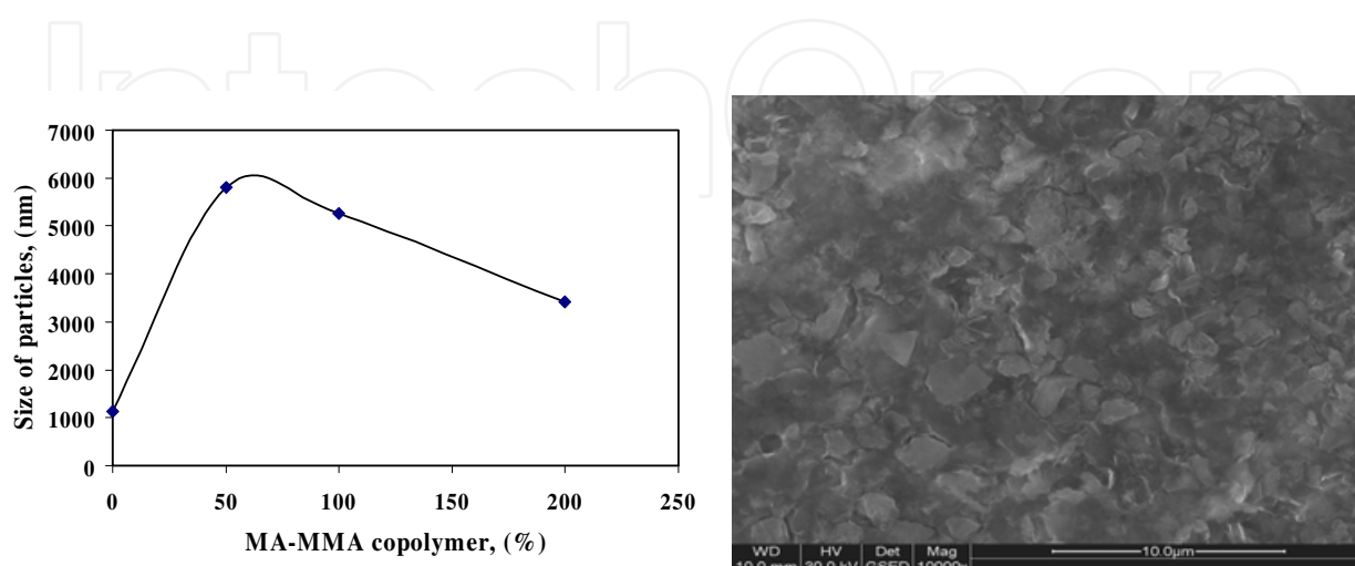
Fig. 5. Particle size and morphology for PB/ MA-MMA binary nanocomposites.
