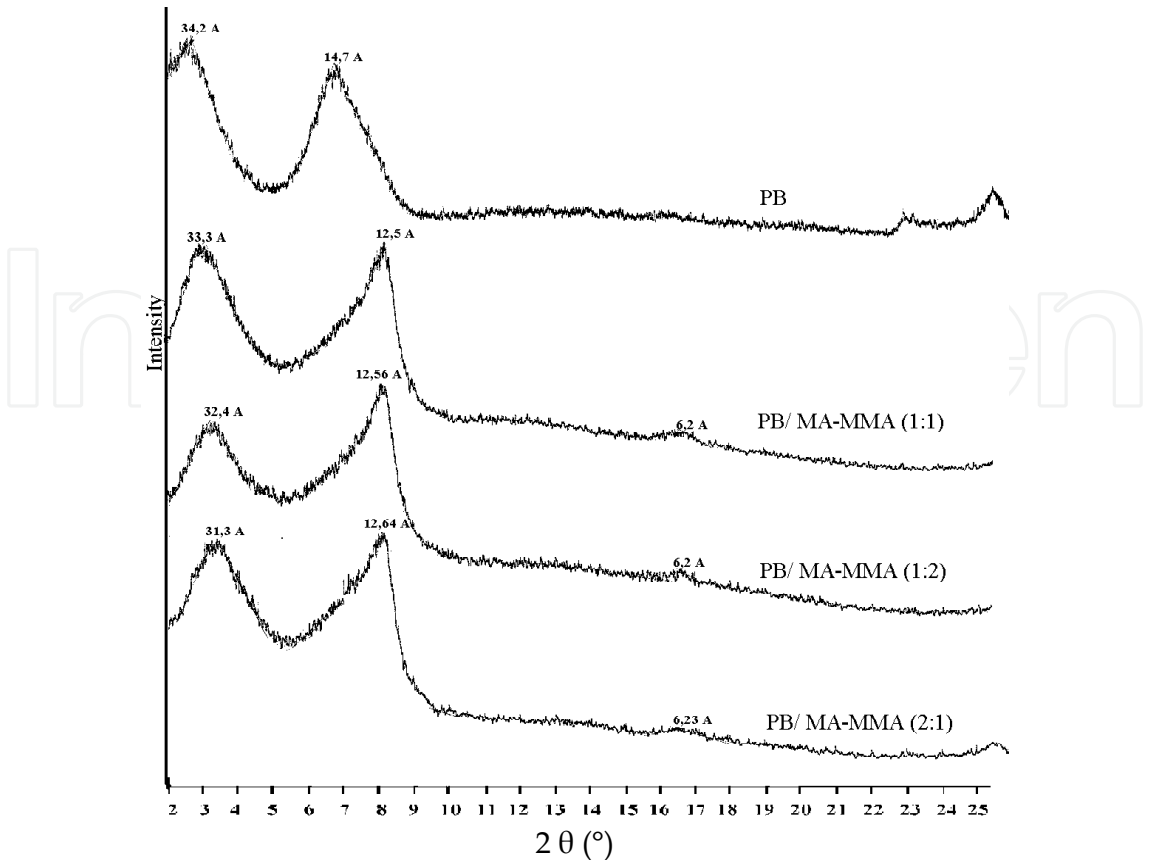
Fig. 7. X-ray diffractions for PB/ MA-MMA nanocomposites at different ratios.
