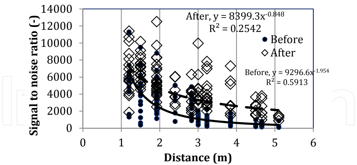
Fig. 9. Signal to noise ratio vs. propagation distance for different repair stages.
