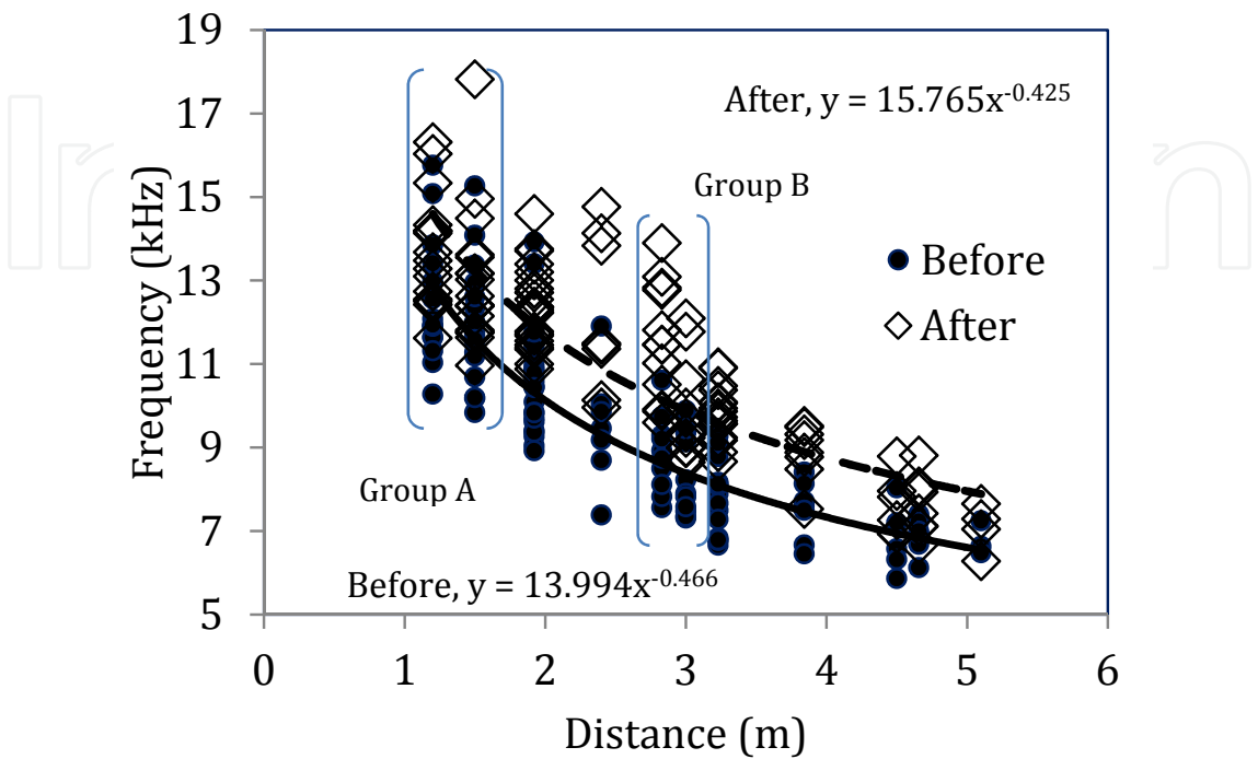
Fig. 7. Central pulse frequency vs. propagation distance for different stages of repair.
