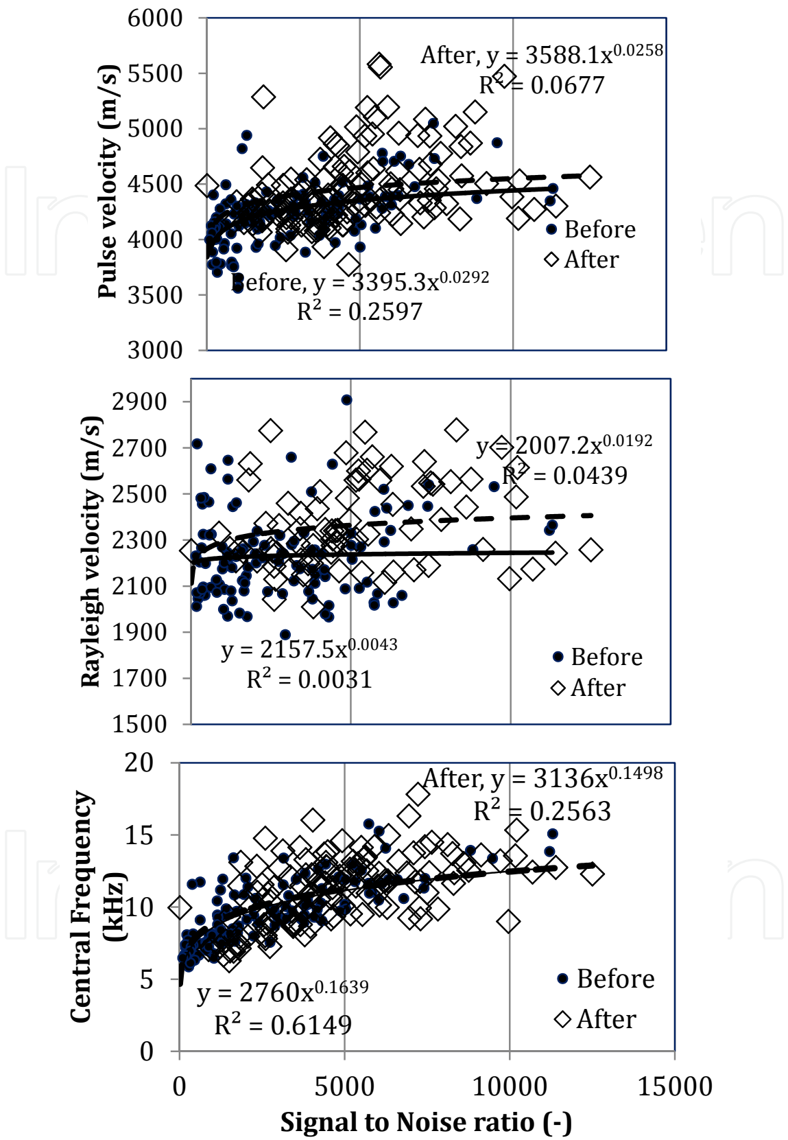
Fig. 8. Wave parameters vs. signal to noise ratio (a) pulse velocity, (b) Rayleigh velocity, (c) central frequency.
