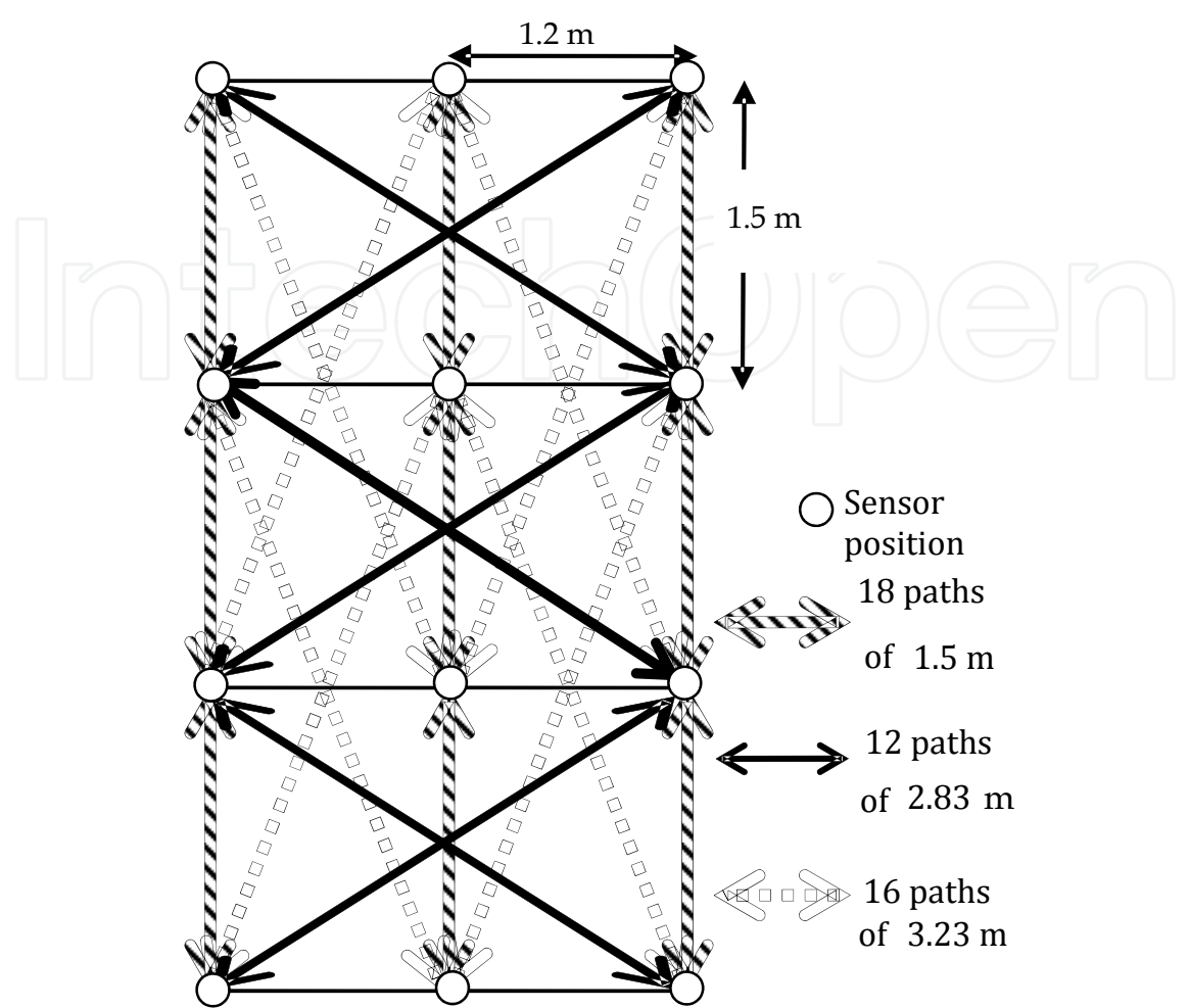
Fig. 2. Pattern of wave measurements and examined wave paths on concrete surface.
