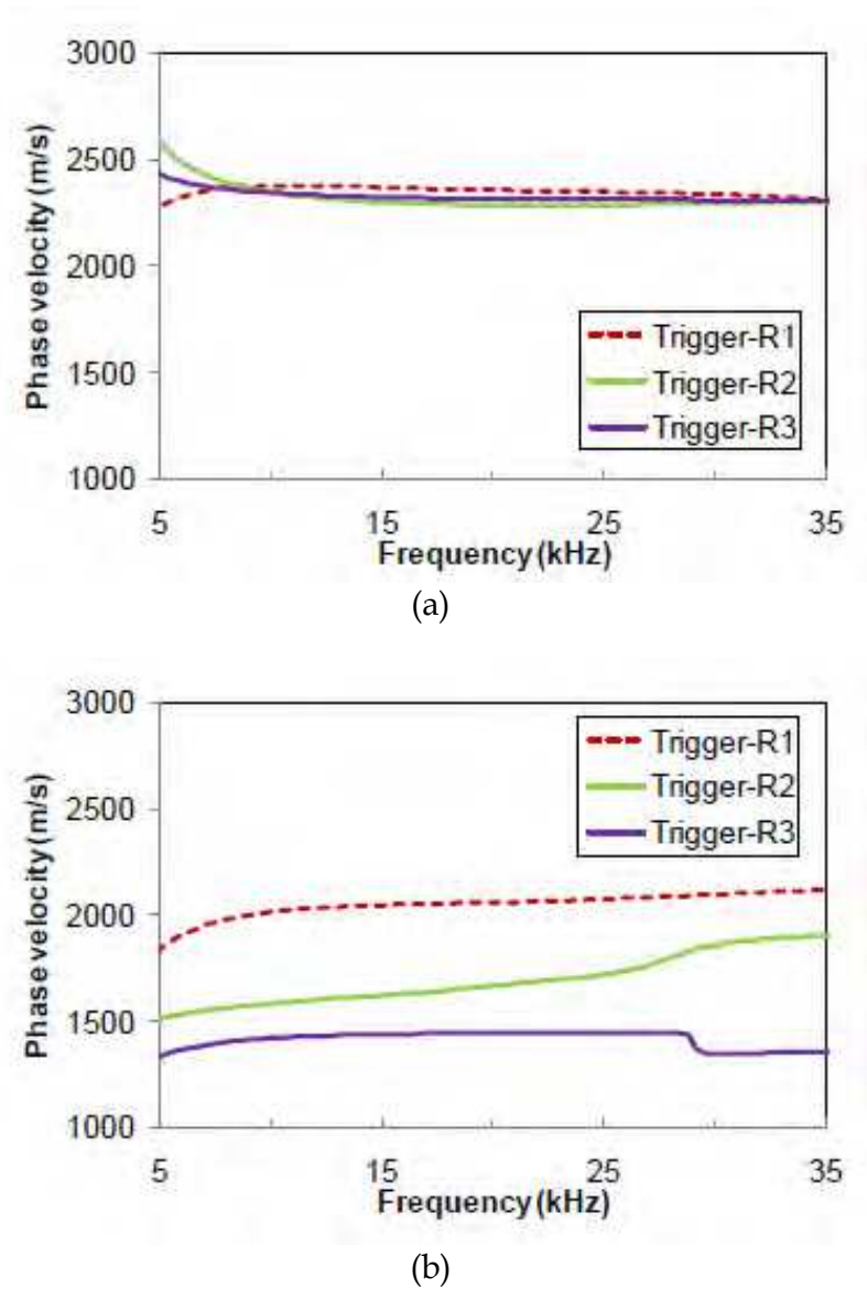
Fig. 16. Dispersion curve computed for data by excitation frequency of 20 kHz, (a) homogeneous concrete and (b) horizontal crack at 50 mm from top
