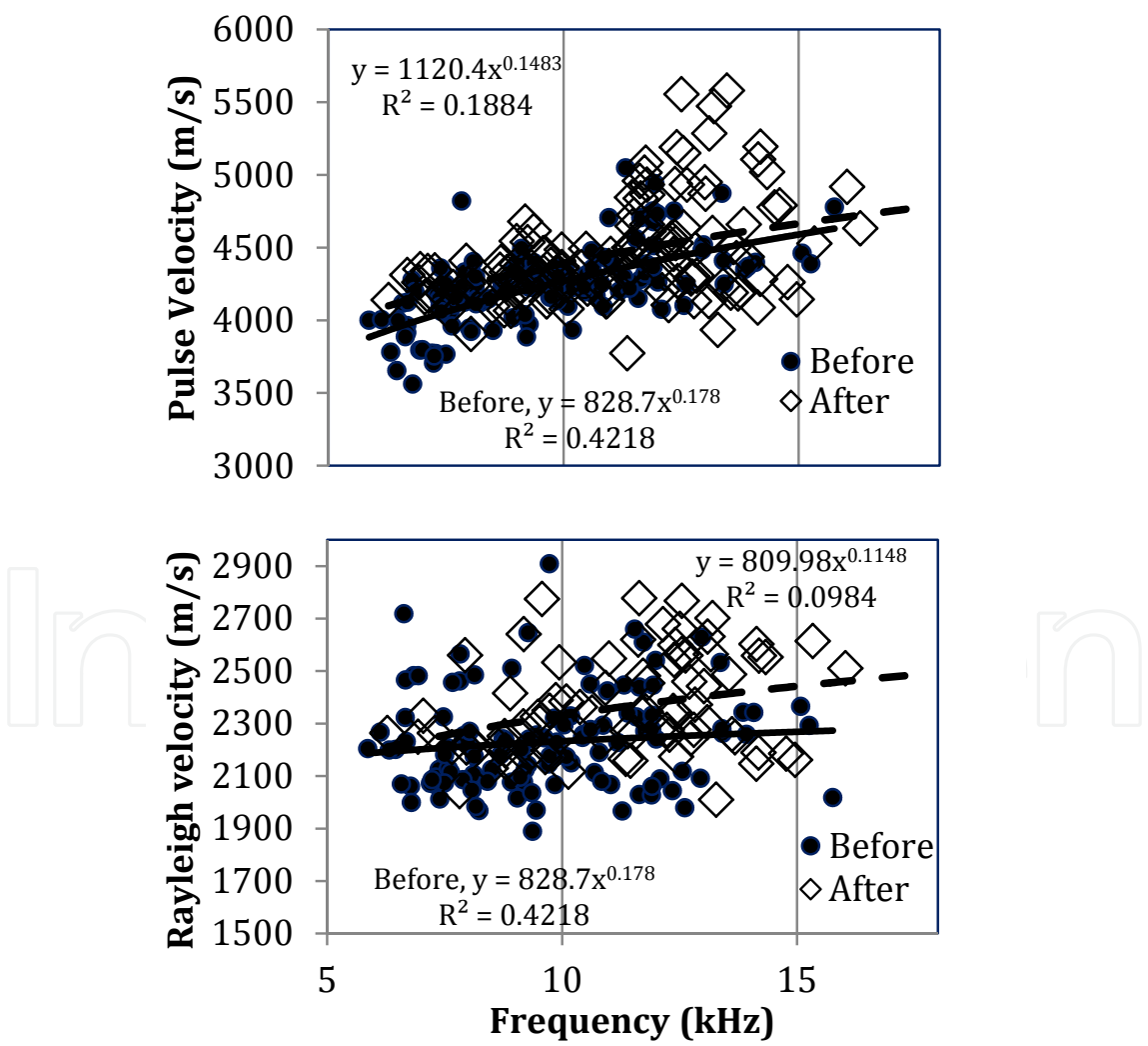
Fig. 10. Pulse (a) and Rayleigh (b) velocity vs. frequency for the total population of measurements.
