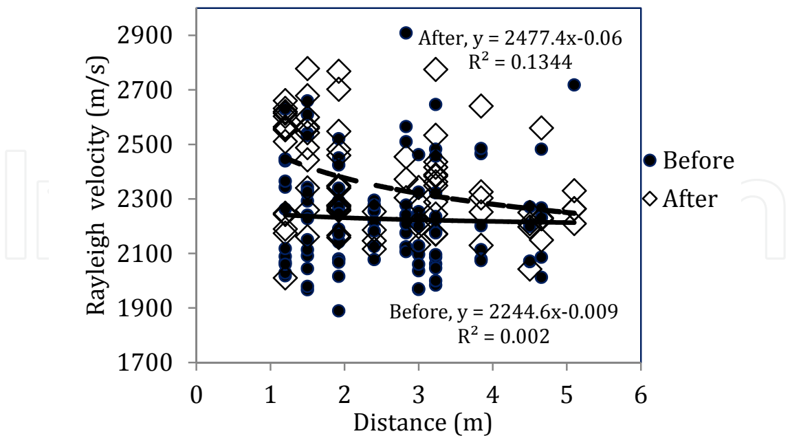
Fig. 5. Rayleigh velocity vs. propagation distance for different stages of repair.
