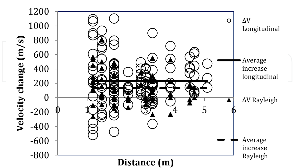
Fig. 6. Difference of velocity between before and after repair for all measurement points.
