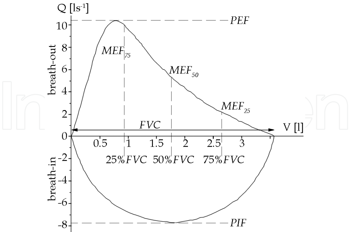
Fig. 5. The spirometric parameters defined on the basis of flow-volume curve Q(V) .
