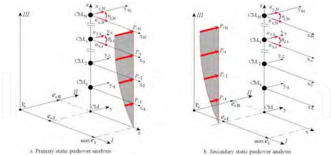
Fig. 4. Spatial Asymmetric Multi-storey System. Primary and Secondary pushover analysis.
