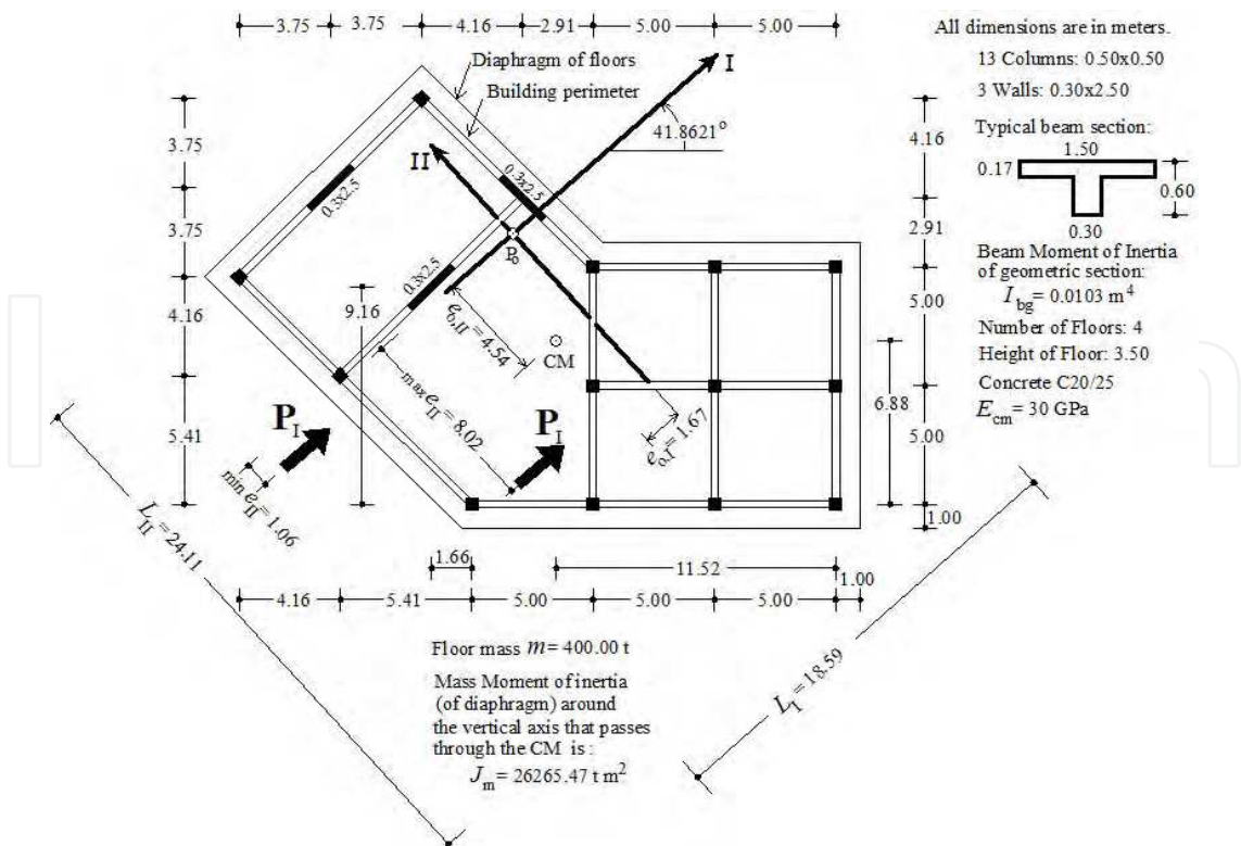
Fig. 1. Typical plan of an asymmetric four-storey r/c building.
