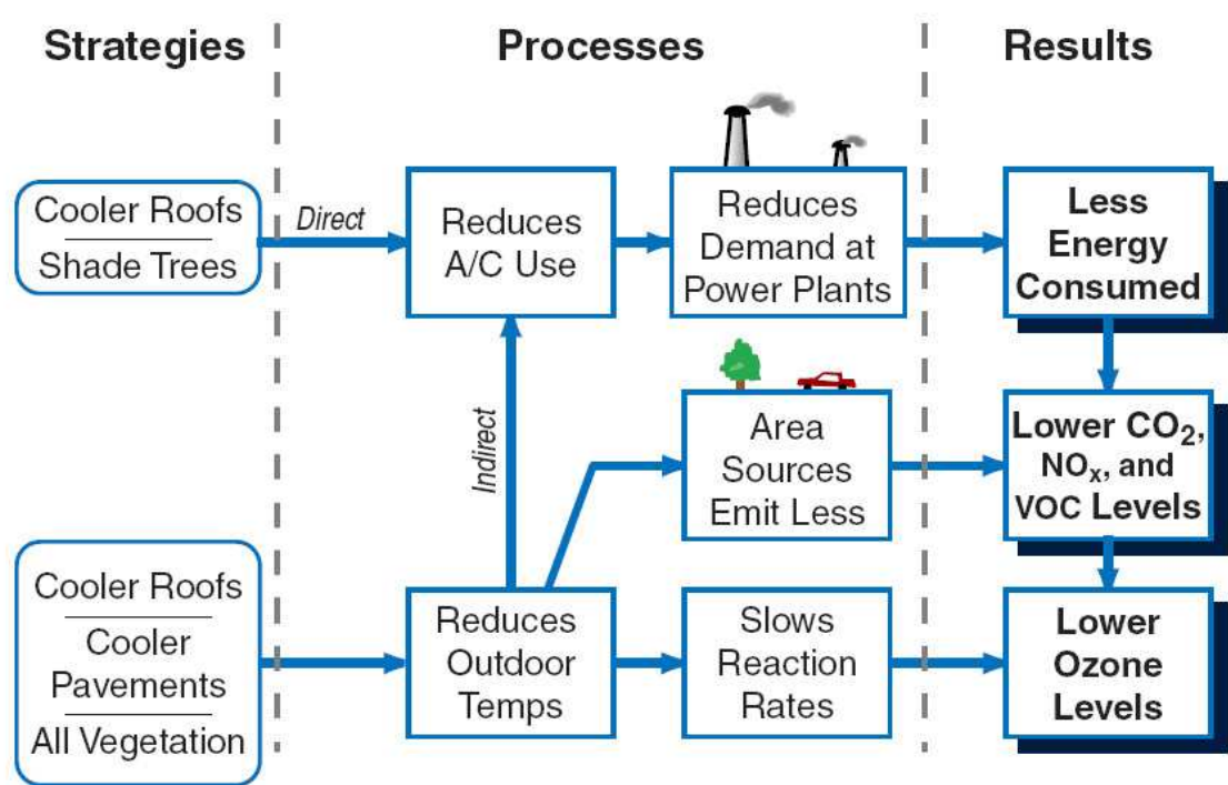
Fig. 11. Direct and direct effects of increasing the albedo of cities (Source: H. Akbari, 2009)
