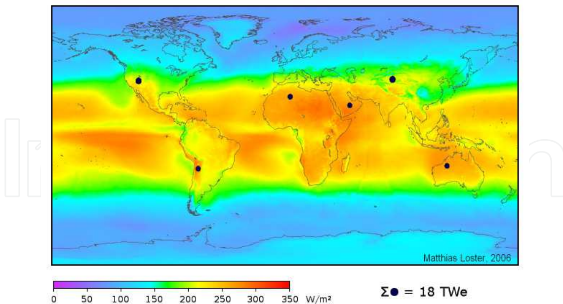
Fig. 3. Solar radiation intensity (Source: http://www.ez2c.de/ml/solar_land_area )
