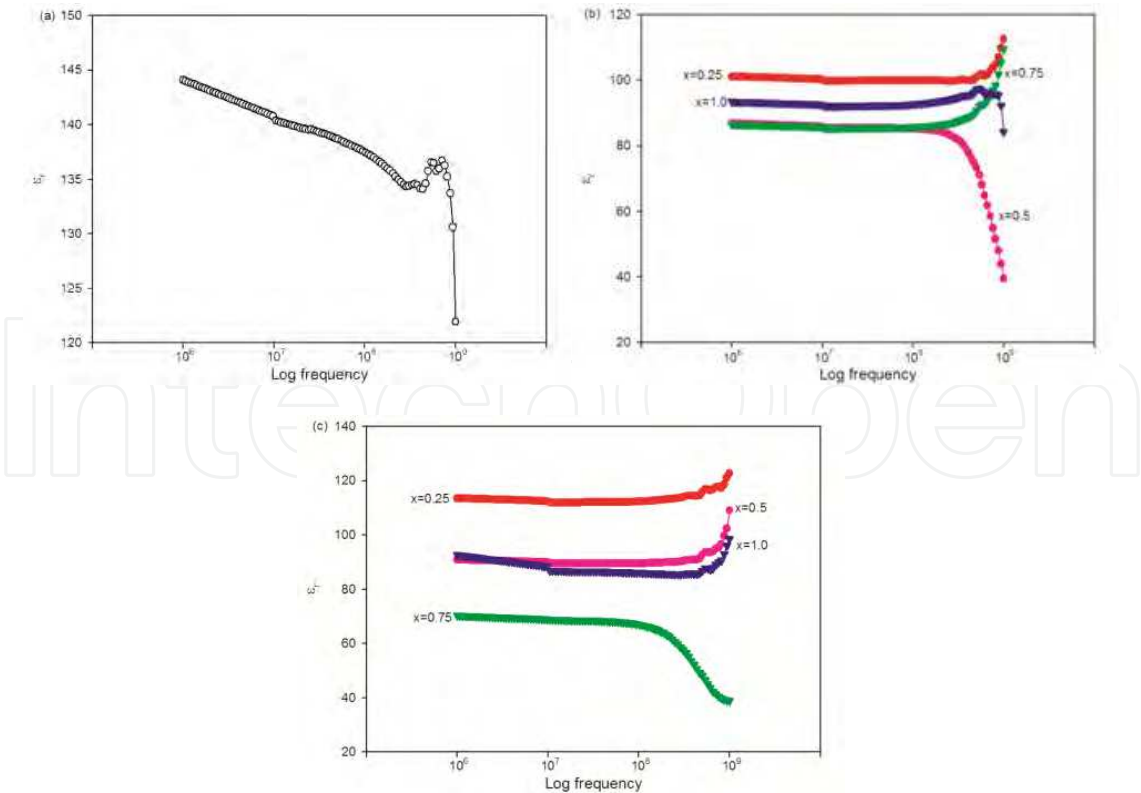
Fig. 11. Dielectric constant, \epsilon_r of (a) BTO, (b) BSmT and (c) BPrT measured at high frequency range at room temperature.
