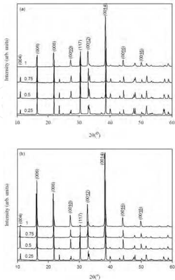
Fig. 7. XRD patterns of (a) BSmT and (b) BPrT ceramics sintered at 1100°C for 3 hour.
