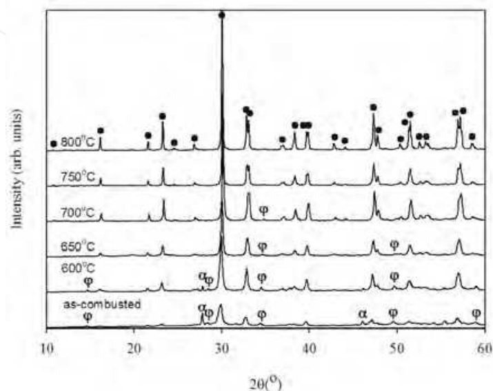
Fig. 2. XRD patterns of BTO powders calcined at different temperatures for 3 hour. ●:Bi 4 Ti 3 O 12 or BTO; α:Bi 7.7 Ti 0.3 O 12.16 or BTO7.7; φ:Bi 2 Ti 2 O 7 or BTO2.
