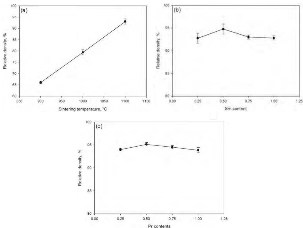
Fig. 9. Relative density of (a) BTO at different sintering temperatures, (b) BSmT with different \text{Sm}^{3+} contents and (c) BPrT with different \text{Pr}^{3+} contents; sintered at 1100°C.
