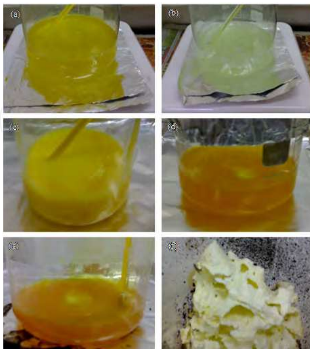
Fig. 1. Evolution of (a) Bi-Ti precursor (b) Pr precursor (c) Bi-Ti precursor stirred at 40°C for 2 hour (d) Bi-Ti precursor heated at 90°C (e) viscous gel and (f) as-combusted powder.
