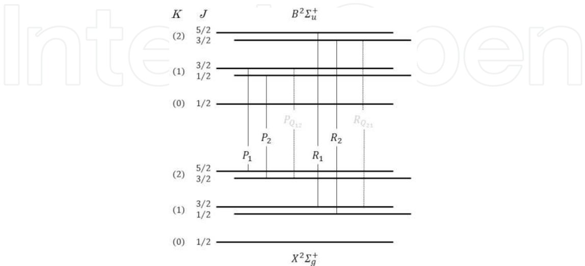
Fig. 9. Transition scheme of N 2 + 1NS. Those indicated in thin lines are negligibly weak.
