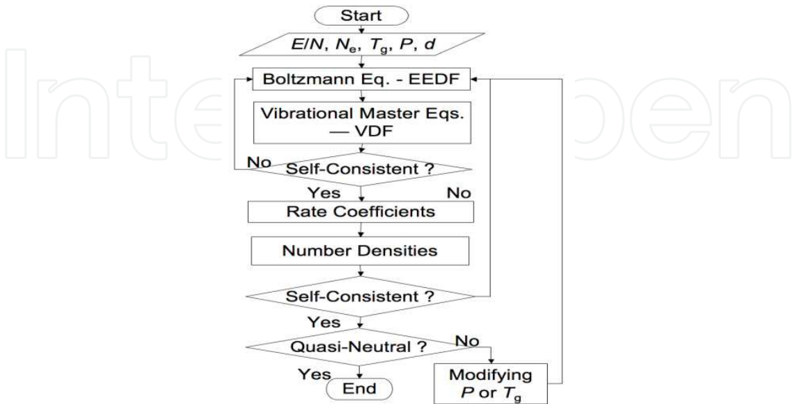
Fig. 14. Flow chart of the numerical procedure (Akatsuka et al., 2008; Ichikawa et al., 2010).
