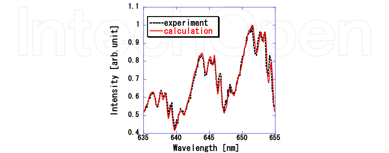
Fig. 7. Example of comparison between 1PS ( \Delta v = 3 ) spectra calculated theoretically and measured experimentally, assuming T_V = 0.65 eV and T_R = 0.15 eV (Sakamoto et al., 2007).
