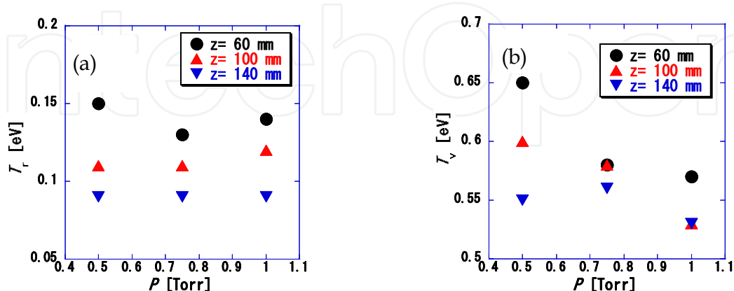
Fig. 8. (a) Rotational and (b) vibrational temperatures of B\ ^3\Pi_g state of N_2 plasma measured experimentally, generated in the apparatus schematically shown in Fig. 3 ( \Delta v = 3 , v' = 7, 8, 9 ) (Sakamoto et al., 2007).
