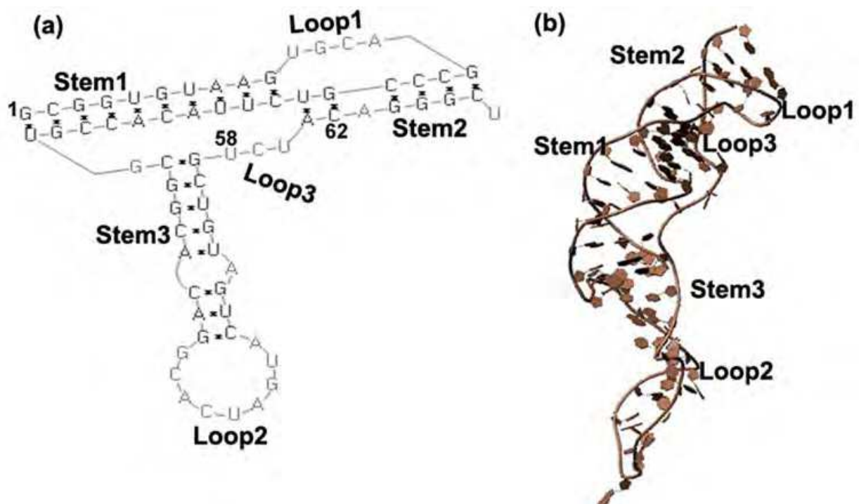
Fig. 4. A) 2-D diagram of the SARS pseudoknot structure. B) 3-D model determined by molecular dynamics simulation. Reprinted with permission from Park et al., 2011, Identification of RNA Pseudoknot-Binding Ligand That Inhibits the -1 Ribosomal Frameshifting of SARS-Coronavirus by Structure-Based Virtual Screening. Copyright 2011 American Chemical Society.
