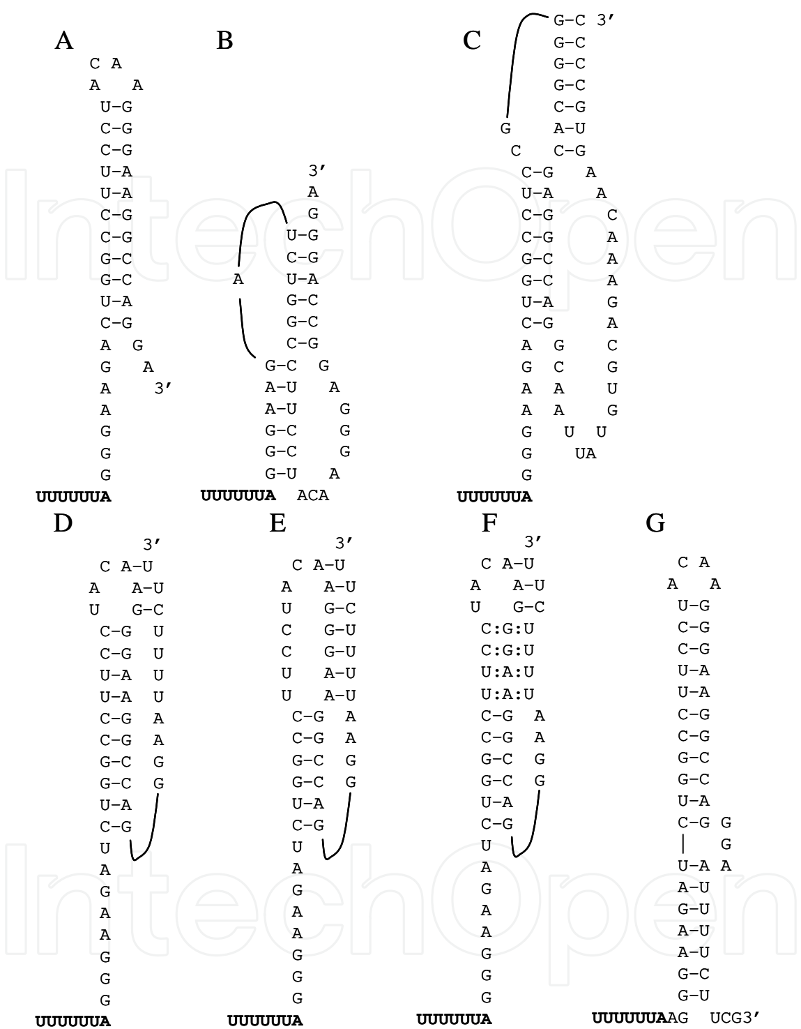
Fig. 3. Different stimulatory elements reported for HIV frameshift signals. There are some minor sequence variations between the subtypes. The stem-loop structure proposed by Jacks et al., (1988a) and pseudoknot proposed by Du et al., (1996) are shown in panels A and B respectively. Panel C shows the pseudoknots described by Baril et al., (2003) for group O isolates. Panels D and E show two pseudoknots proposed by Taylor et al., (1994) and panel F shows the pseudoknot described by Dinman et al., (2002) using the same sequence. The extended stem-loop structure with a 5'-ACAA-3' tetraloop described by Dulude et al., (2002) is shown in panel G.
