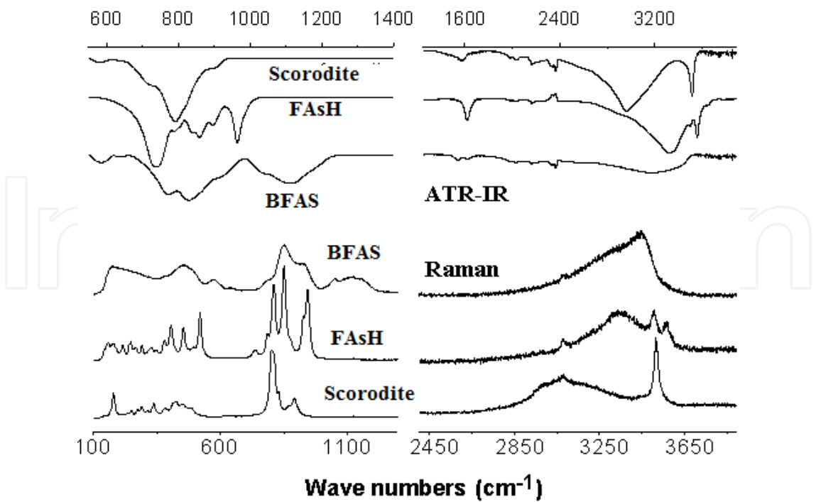
Fig. 5. ATR-IR (top) and Raman of the three main arsenate phases produced in our studies. These were Scorodite, Ferric Arsenate sub-Hydrate and Basic Ferric Arsenate Sulfate. Note the much richer IR structure observed in the arsenate and hydroxyl stretching region for these phases (e.g. Type 1 = FAsH) in comparison to that of the Transmission mode used in Figure 4 above.
