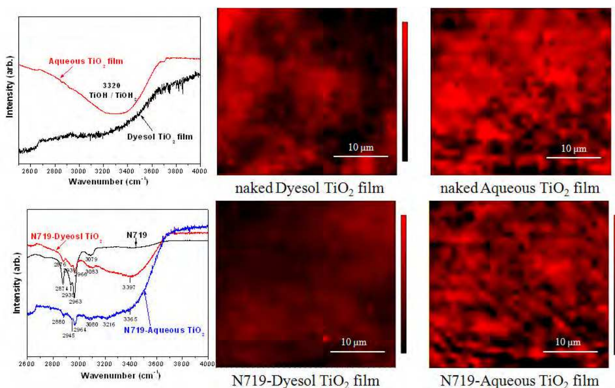
Fig. 12. ATR-IR spectra (Hydroxyl region) and corresponding images of the pure \text{TiO}_2 substrates (Dyesol and Aqueous) and that of the adsorbed N719- \text{TiO}_2 system. (Lee et al. 2010, 2011b)
