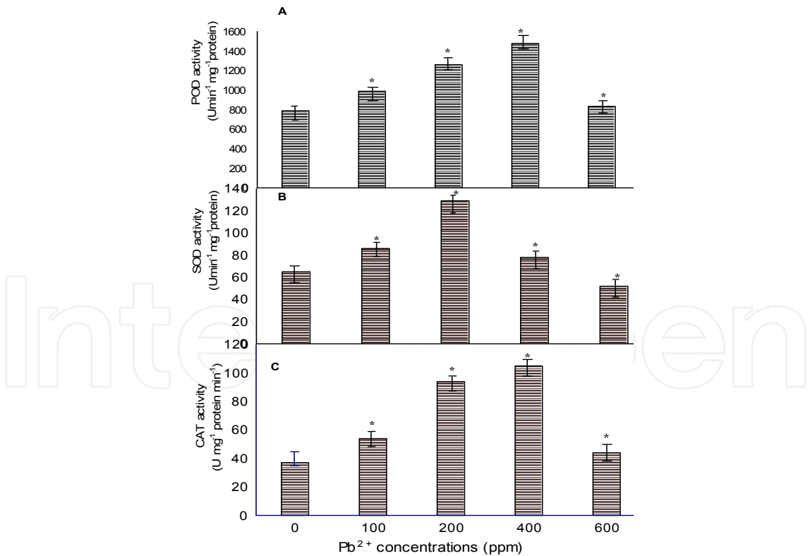
Fig. 6. Antioxidant enzyme activities POD (A), SOD (B) and CAT(C) of Lepidium sativum leaves subjected to various concentrations of Pb 2+ . Each value represents the mean ±SE of five replicates. Significant differences (P<0.05) between treatments according to LSD test are shown by an asterisk (Ibrahim & Bafeel, 2011).
