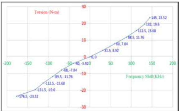
Fig. 44. The experimental results between the torque and frequency shift.
