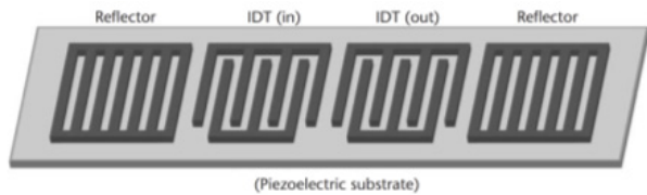
Fig. 20. The two-port SAW resonator (Humberto Campanella, 2010).
