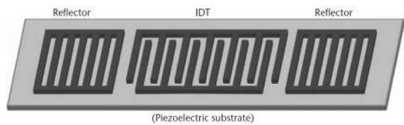
Fig. 18. The one-port SAW resonator (Humberto Campanella, 2010).
