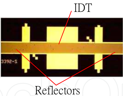
Fig. 28. The microimage of the SAWR's die.
