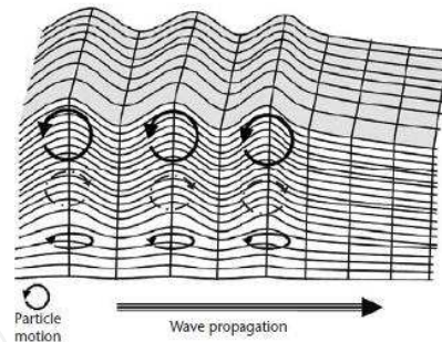
Fig. 1. Rayleigh wave propagation. (Auld ,1990).
