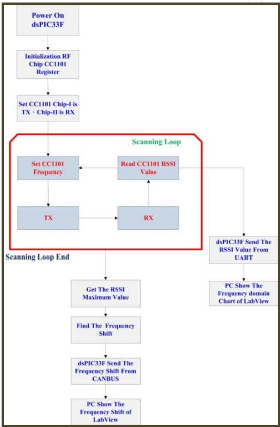
Fig. 42. The flow chart of the dSPIC 33F program.
