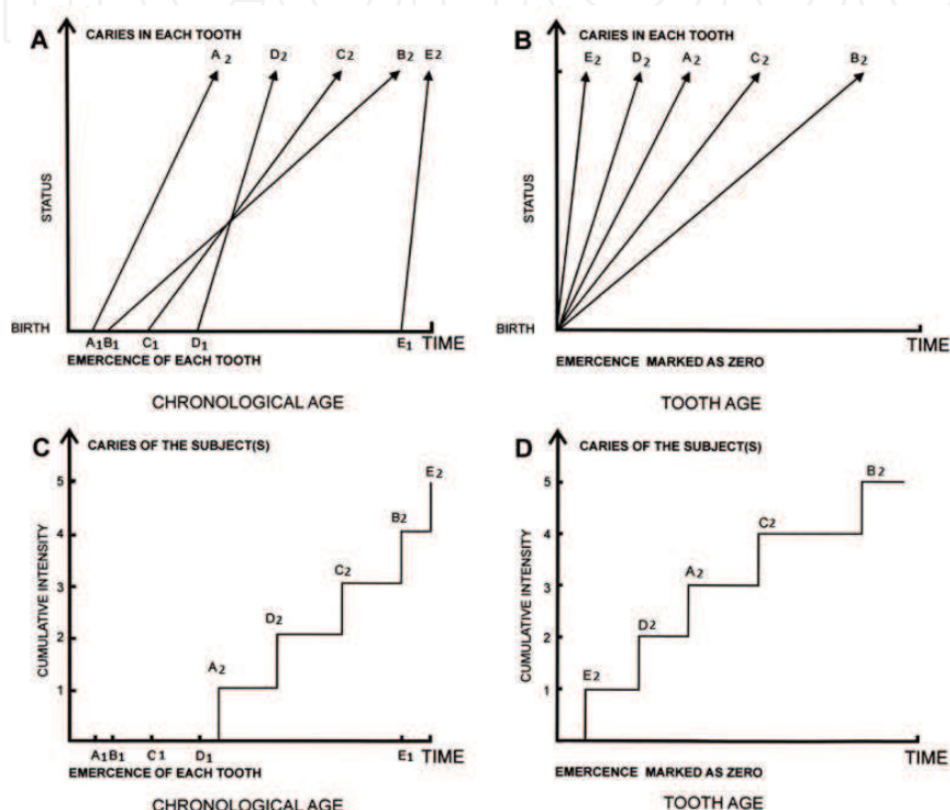
Fig. 3. The principle of time to event analysis
