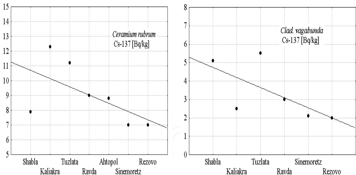
Fig. 11. 137 Cs content in macroalgae – local variations
