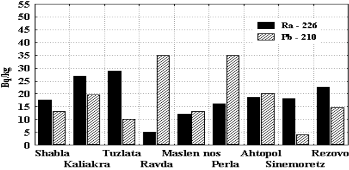
Fig. 12. Mean 226 Ra and 210 Pb content (Bq/kg) in Ceramium rubrum
