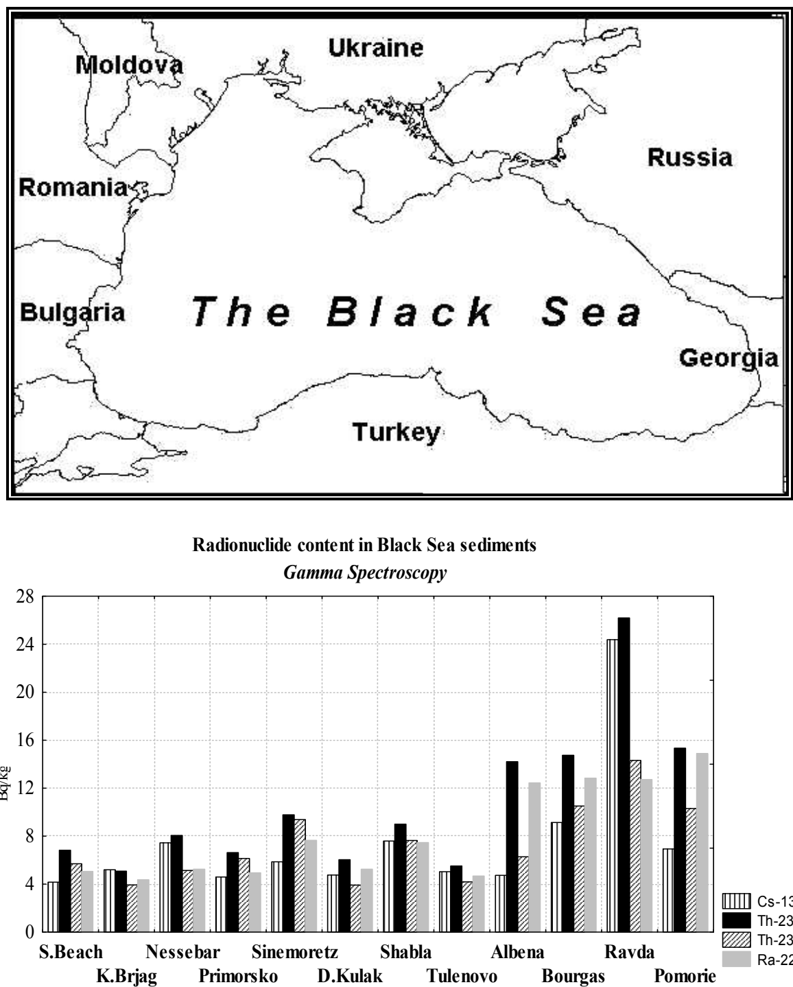
Fig. 2. Nuclide content in sand sediments along the Bulgarian coast
