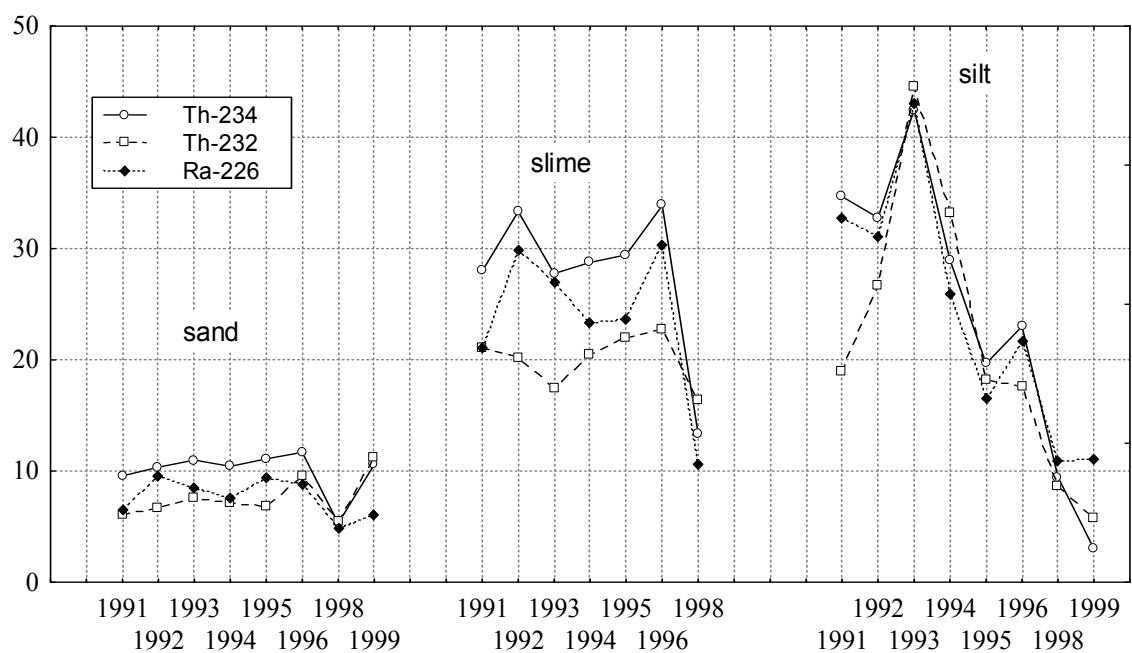
Fig. 5. Natural nuclide content (Bq/kg) in Black sea sediments in the 1991 – 1999 period Samples were taken from deep sediments (56 – 155 m) from the Bulgarian territorial waters plus two samples at maximal depth 2040 m and also were measured for radionuclide content.
