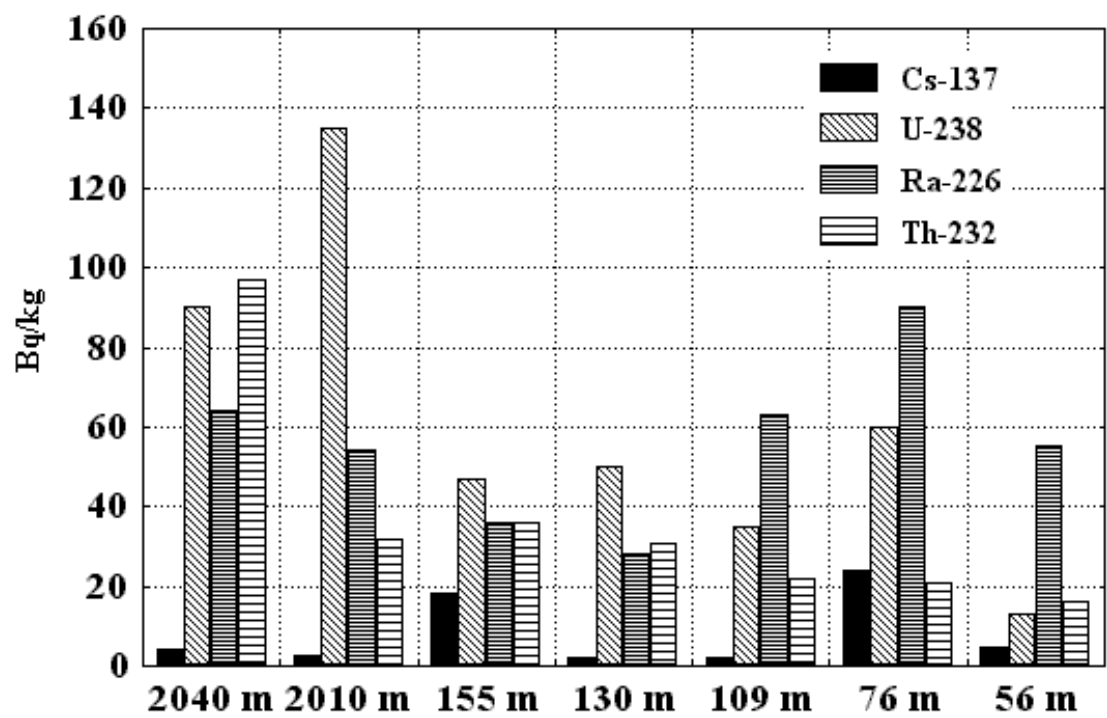
Fig. 6. Mean nuclide content in deep-sea sediment samples
