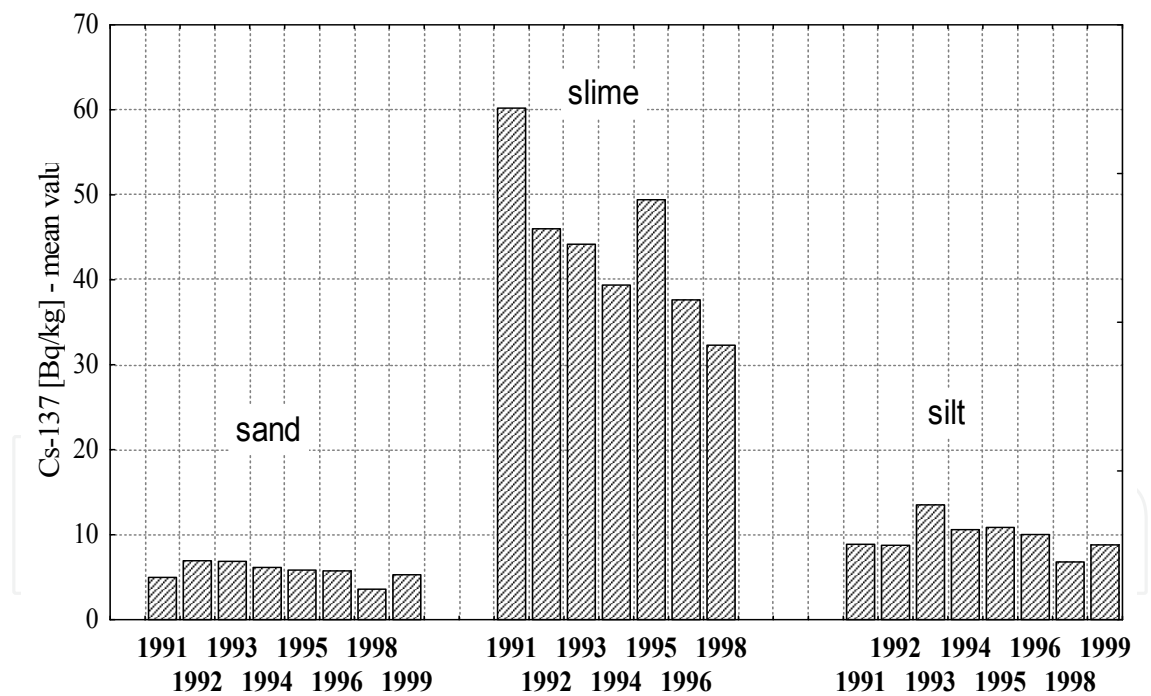
Fig. 4. Mean 137 Cs content in sediments during the period 1991 - 1999
