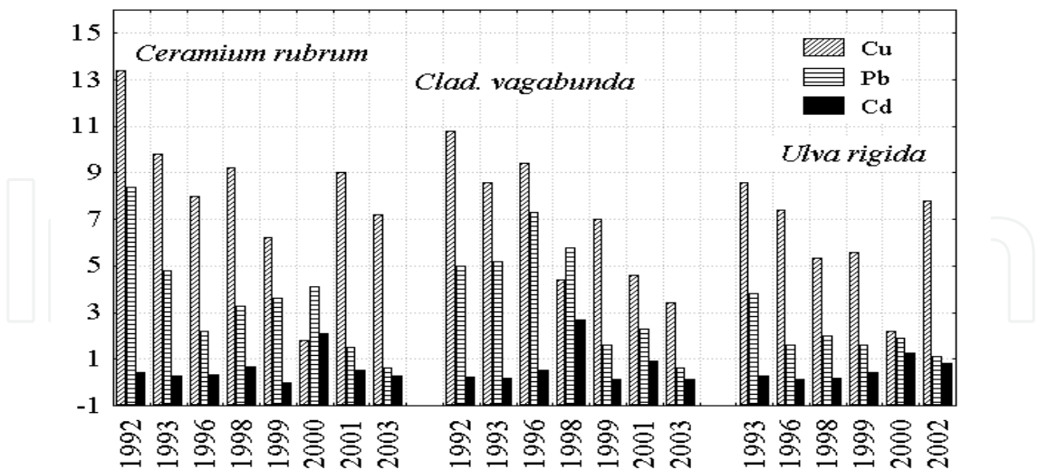
Fig. 13. Seasonal variations of HM concentrations (mg/g) in three alga species
