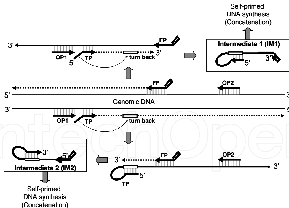
Fig. 2. Formation of intermediate products in the initial step of the SmartAmp reaction. The priming events of the SmartAmp reaction generate two intermediates (i.e., IM1 and IM2).
