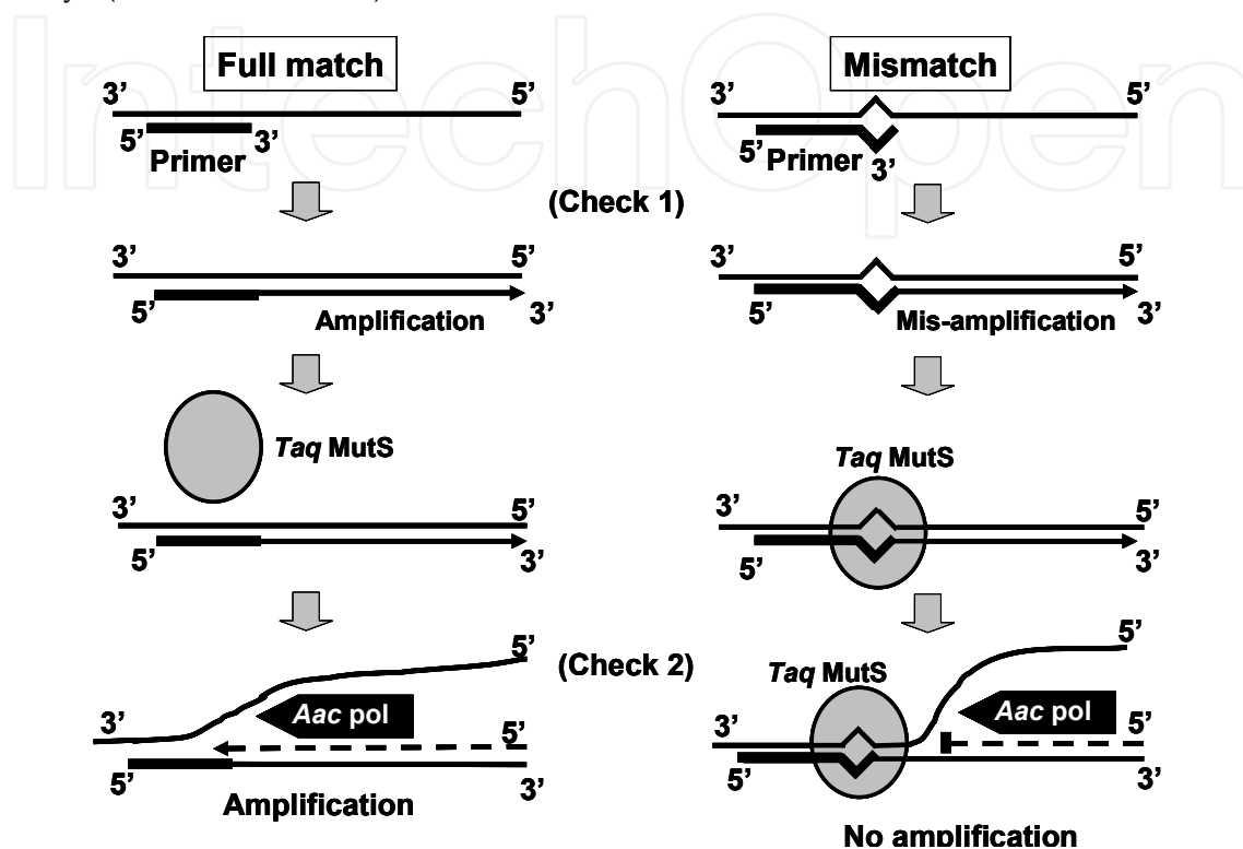
Fig. 4. The mechanism of allele discrimination as exercised by Taq MutS. SNP typing with a wild-type allele detection primer, using the wild-type allele (left) and the mutant-type allele (right) as templates. The wild-type allele detection primer is designed to encompass the SNP nucleotide site at each 3'-position. Amplification is not allowed when the primer mismatches with the mutant-type allele (Check 1). If check 1 fails, Taq MutS strongly binds to mismatched nucleotides and Aac DNA polymerase can not strand-displace or extend the newly synthesized strand (Check 2).
