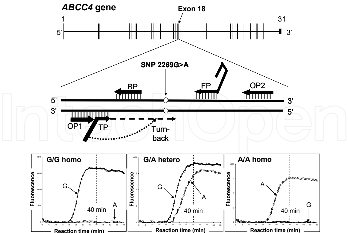
Fig. 8. Schematic illustration of the human ABCC4 gene located on chromosome 13q32.1. The SNP 2269G>A that resides in exon 18 was detected by the SmartAmp method.
