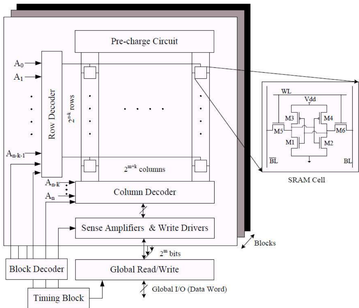
Fig. 1. SRAM architecture.
