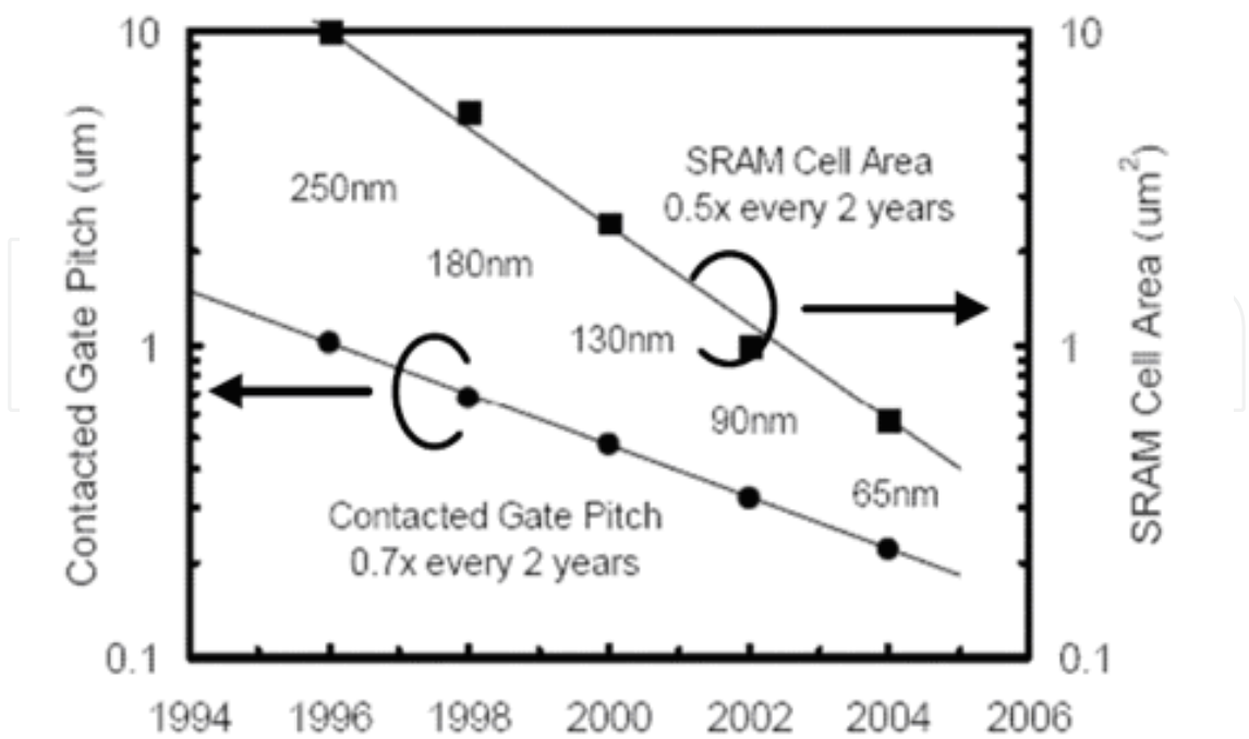
Fig. 9. SRAM cell size has been scaling at ~0.5 x per generation.
