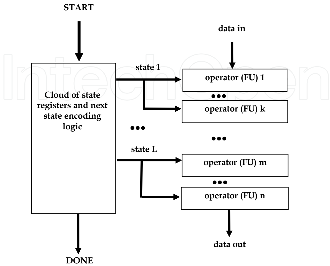
Fig. 5. Massively-parallel microarchitecture generation option.
