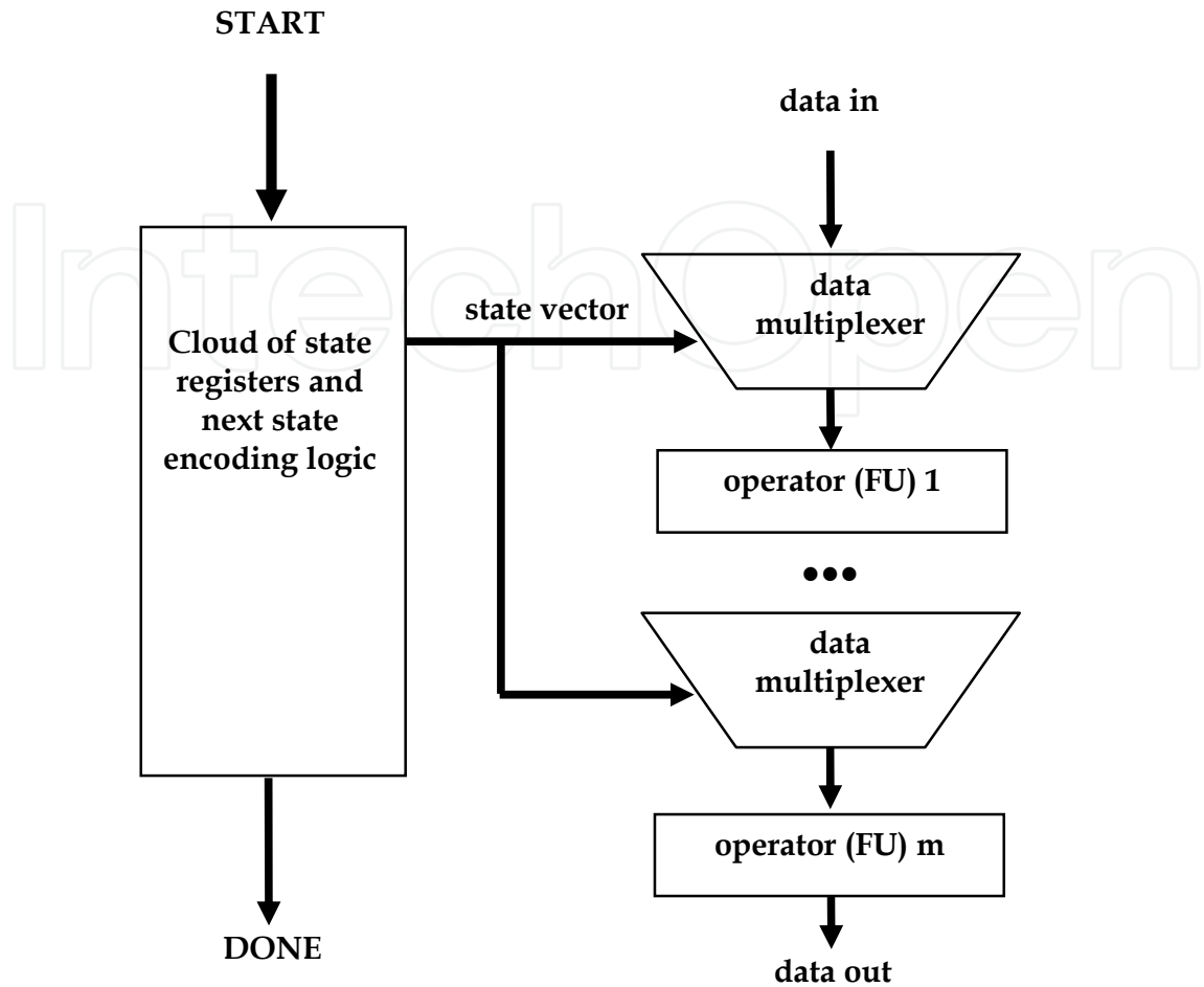
Fig. 6. The traditional FSM + datapath generated micro-architecture option.
