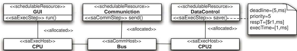
Fig. 3. Architectural Part of the SAV
