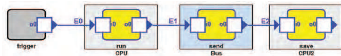
Fig. 6. Representation in SymTA/S
