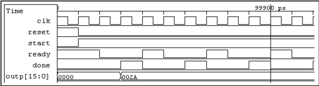
(c) Timing diagram.
