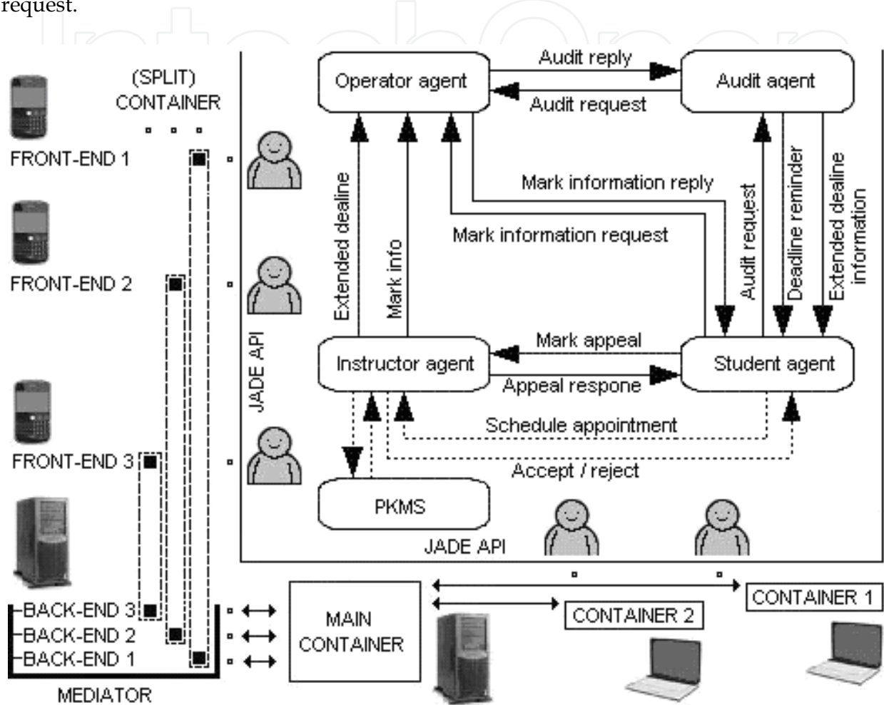
Fig. 5. PKMS specific area module m-learning architecture in context of mobile devices and agent development environment JADE-LEAP
