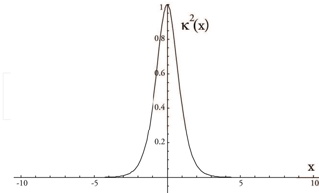
Fig. 5. The curvature \kappa^2 = 1 - \tanh^2(x) .
