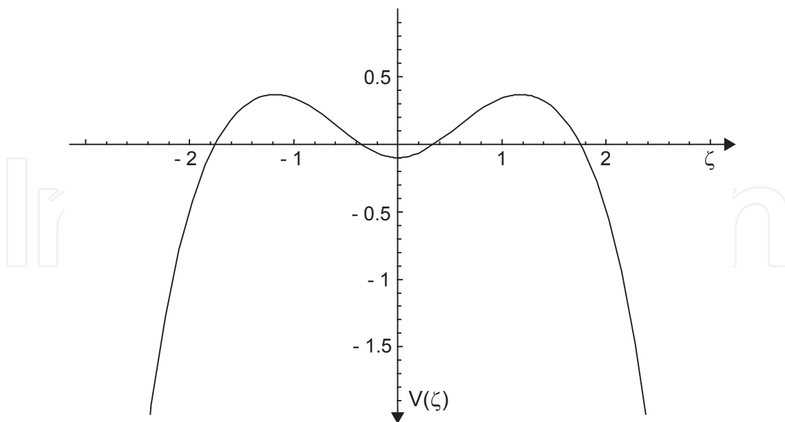
Fig. 2. The inverted double well potential V(\zeta) with m = \pm 1 and \epsilon = 0.1 .
