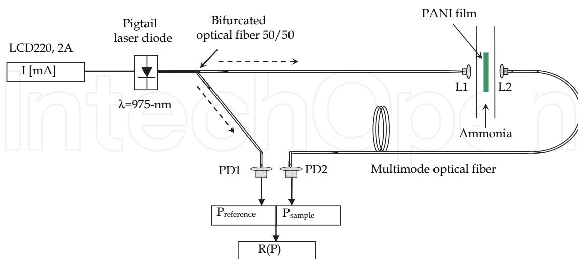
Fig. 8. Laser sensor system for the remote optical detection of ammonia with PANI films employing the optical transmittance ratio technique. (Castrellon-Urbe et al., 2009).
