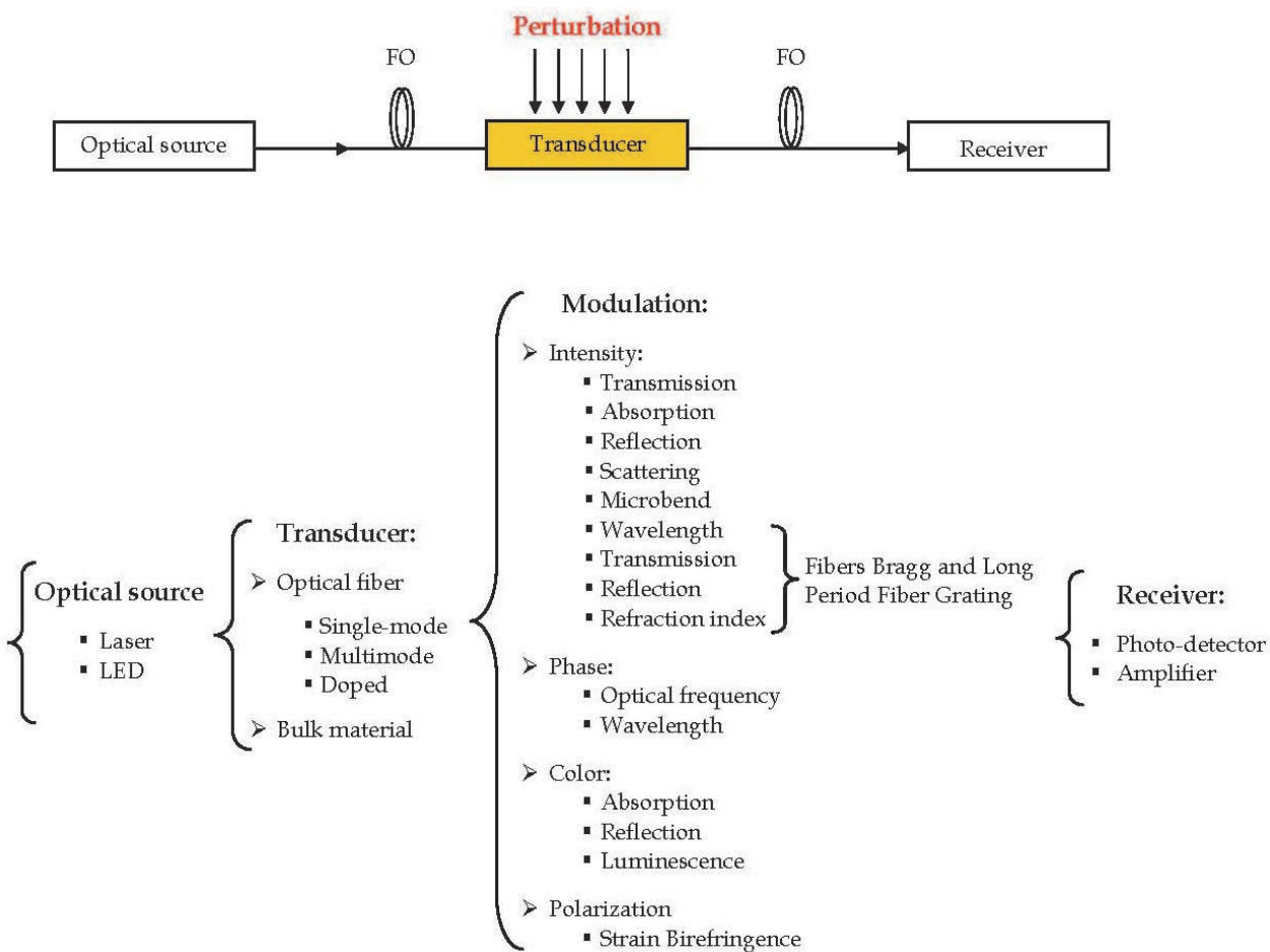
Fig. 3. Basic components of an optical fiber sensor.
