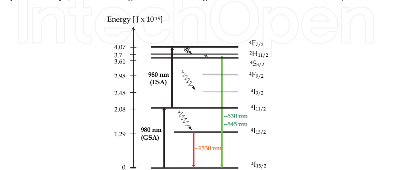
Fig. 5. Erbium energy levels diagram illustrating the excited state absorption (ESA) and the up-conversion fluorescence process. (Castrellon-Uribe & Garcia-Torales, 2010).
