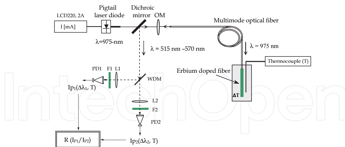
Fig. 6. Experimental setup of the erbium-doped silica fiber sensor for remote temperature measurements, employing the up-conversion fluorescence intensity ratio technique. (Castrellon-Urbe & Garcia-Torales, 2010).
