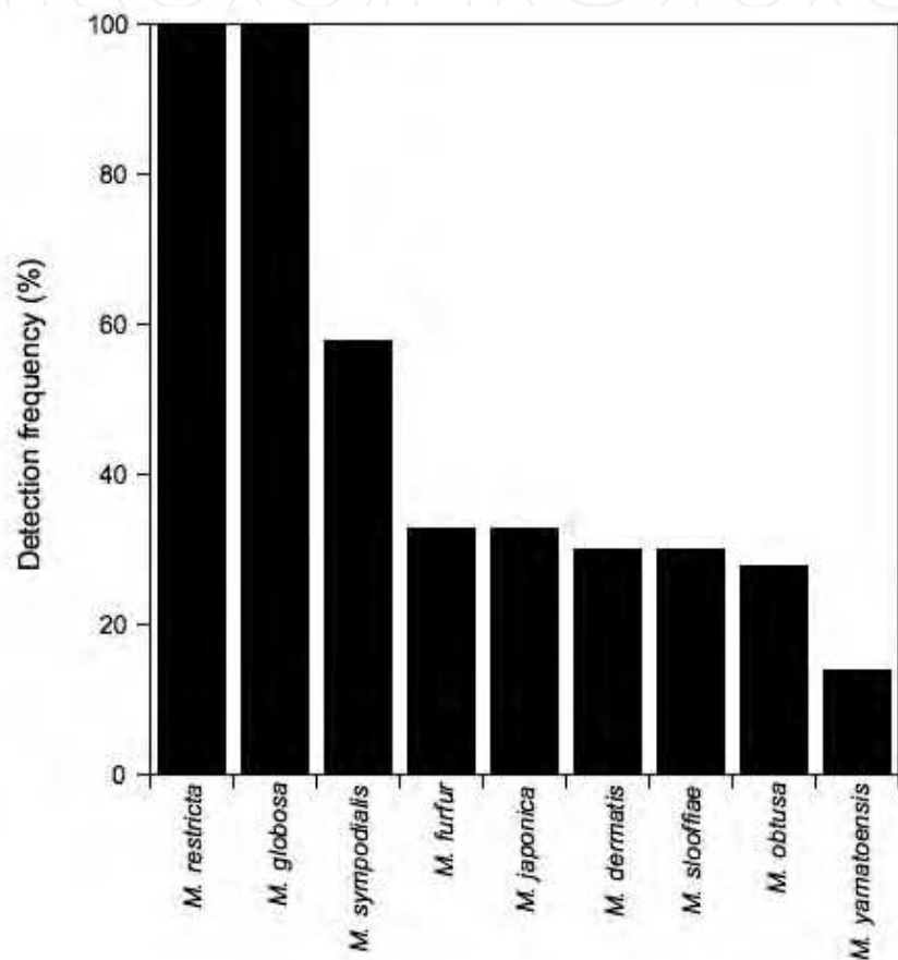
Malassezia DNA was detected by nested PCR assay with species-specific primers Fig. 2. Colonization frequency of Malassezia in the scale of patient with atopic dermatitis
