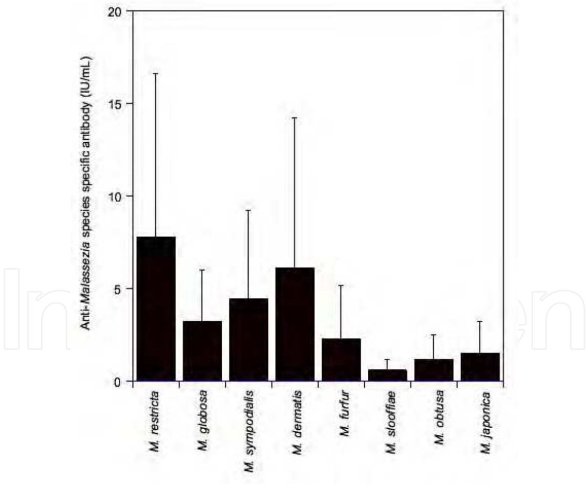
Fig. 7. The species-specific IgE values of eight Malassezia species in sera from patients with atopic dermatitis determined using an ELISA.
