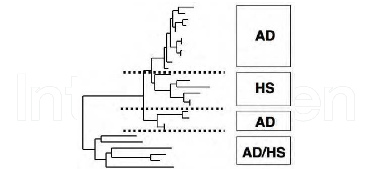
AD, patients with atopic dermatitis; HS, healthy subjects. Fig. 4. Phylogenetic tree of M. globosa colonizing the skin surface of AD patients and healthy subjects based on DNA sequences of the IGS 1 region
