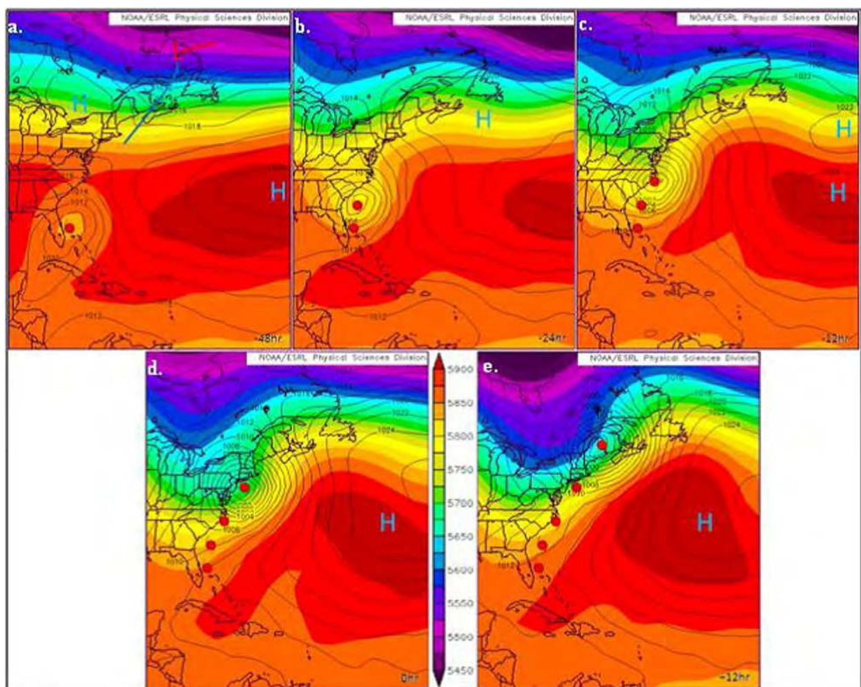
Fig. 8. Composite time series for Hurricanes Carol (August 31, 1954 at 12Z), Edna (September 11, 1954 at 18Z), and Donna (September 12, 1960 at 18Z). Solid contours are SLP (2 hPa intervals) and shaded contours are 500-hPa geopotential heights (50 m intervals). Time series from top left to bottom right are: (a) 48 hours, (b) 24 hours, and (c) 12 hours prior to landfall; (d) during landfall; and (e) 12 hours after landfall.
