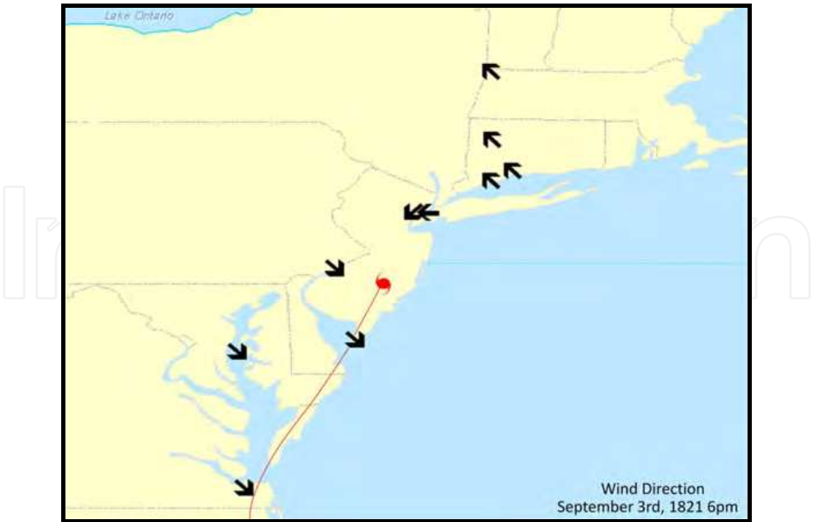
Fig. 10. The approximate location of the 1821 New England Hurricane (New Jersey) and wind direction at ten land locations taken around 22Z on September 3 rd .
