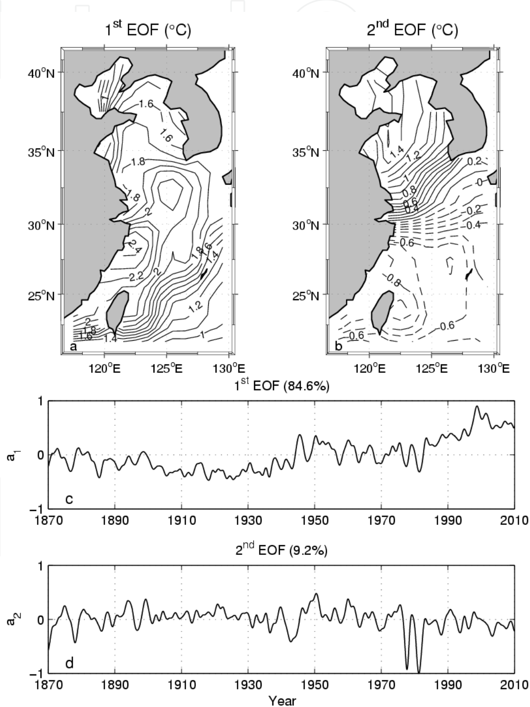
Fig. 9. The spatial and temporal EOF modes of AM. a) The first spatial mode. b) The second spatial mode. c) The first temporal mode. d) The second temporal mode.
