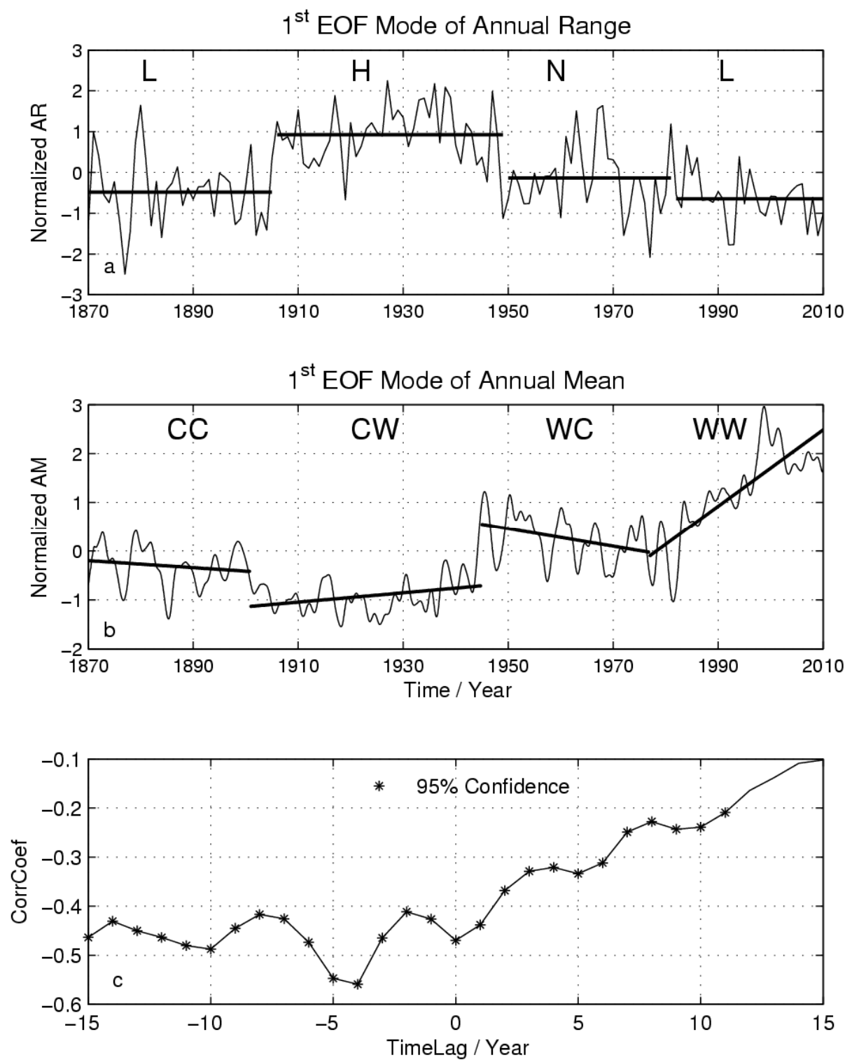
Fig. 10. The regime shifts of SST in the YES. a) The four regimes of in the first EOF mode of AR, L, H and N stand for the low, high and normal variability of AR. b) The four regimes of the first EOF mode of AM, CC, CW, WC and WW stand for the cold regime with a cold trend, cold regime with warm trend, warm regime with cold trend and warm regime with warm trend. c) Correlation coefficient between AR and AM, negative (positive) time lag means that AR lags (leads) AM.
