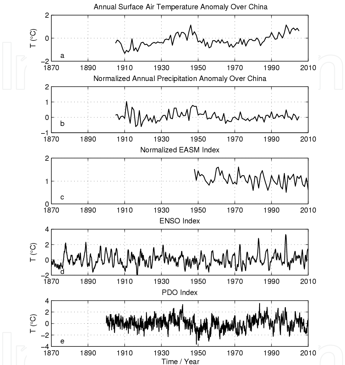
Fig. 2. Time series used to represent regional and global climate. a) Annual surface air temperature anomaly over China (TAC). b) Normalized annual precipitation anomaly over China (PAC). c) EASM Index. d) ENSO index. e) PDO index.
